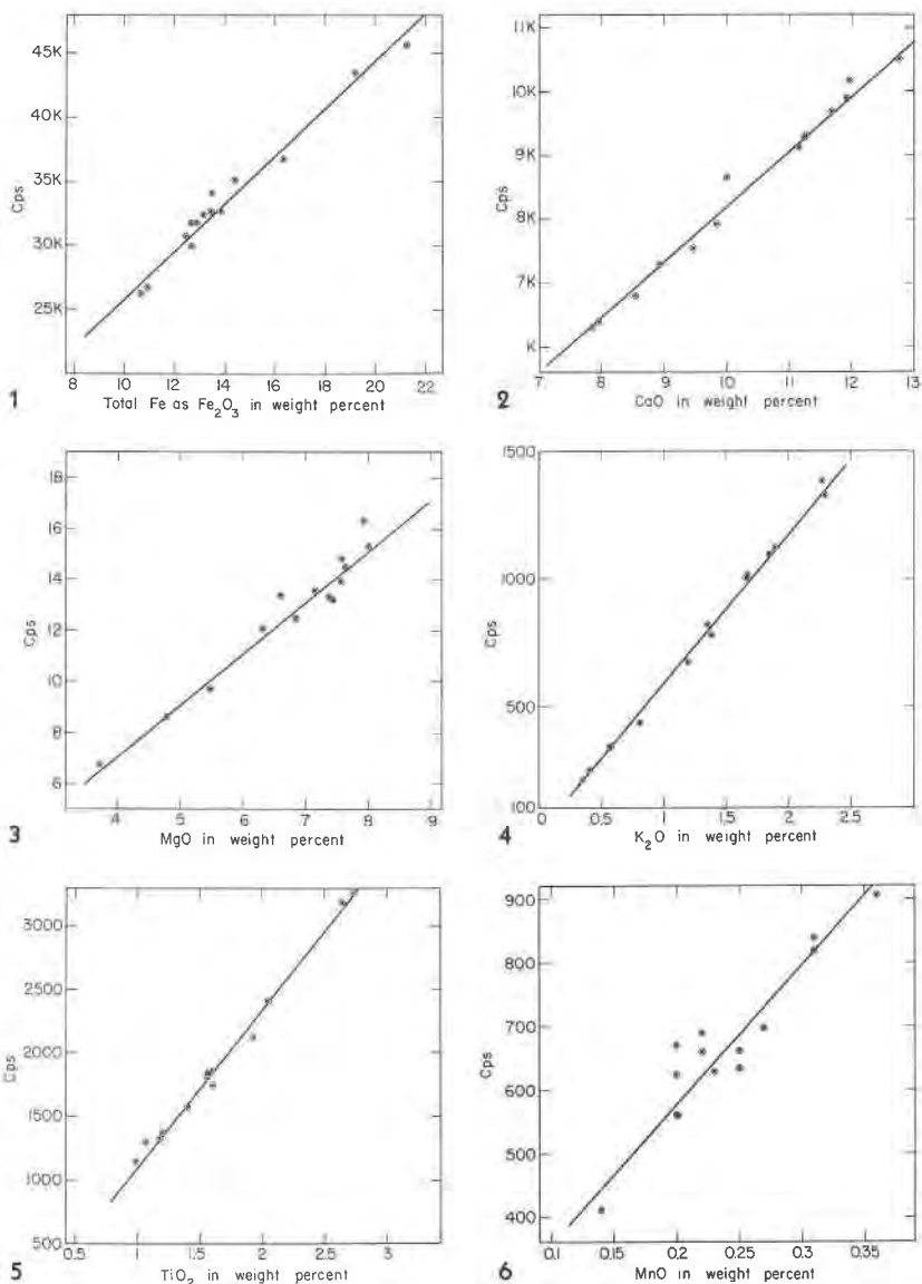
FIGS. 1-6. Calibration curves for fluorescent x-ray analysis.
