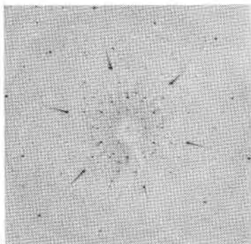
FIG. 1. Davidite, Norway, heated to 960° C. 30° hki0 precession photograph of twin on (5270). Mo-Zr, 28 hours.
