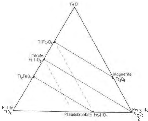
Fig. 6. Concentration triangle for the system \text{FeO}-\text{Fe}_2\text{O}_3-\text{TiO}_2 . Following Gorter (1957), components are formulated so that each has the same number of metal atoms in order that the several mix-crystal series may be represented by parallel lines. Dashed lines show the trends of composition changes with oxidation or reduction.
