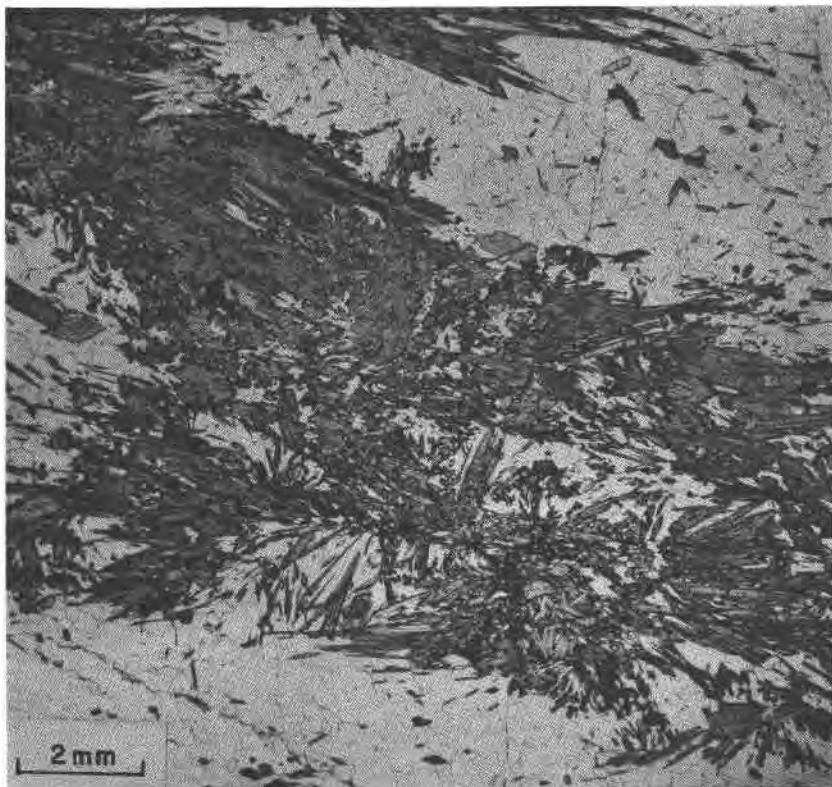
FIG. 2. Sheaf-like cluster of anthophyllite in quartz-oligoclase-anthophyllite schist. Matrix consists of nearly equal amounts of quartz and oligoclase ( Ab_{80} ). The opaque mineral is rutile in part altered to leucoxene. Mitchell Gulch formation, near center sec. 30, T. 49 N., R. 11 E., Fremont County, Colorado. Plane polarized light.
