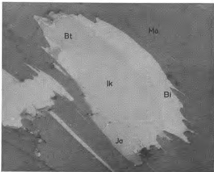
FIG. 2. The association ikunolite-bismuth-bismuthinite-joseite A in molybdenite (Mo). \times 150 .
