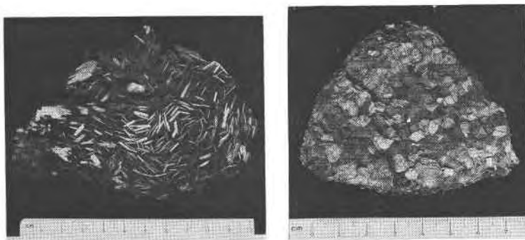
FIG. 5. (Left) Ramsdellite, group of crystals, Lake Valley, New Mexico.
