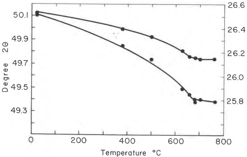
FIG. 5. Thermal expansion of 10% GeO 2 -90% SiO 2 solid solution in terms of 2θ (CuKα) for the 112 and 101 planes.
