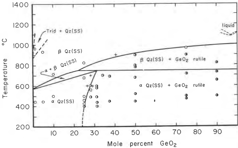
FIG. 2. Phase diagram of the system SiO 2 -GeO 2 based on dry studies and hydrothermal studies at 700 bars. 1 The boundaries determined both by phases and by compositions of Qz (SS) in two-phase fields.
