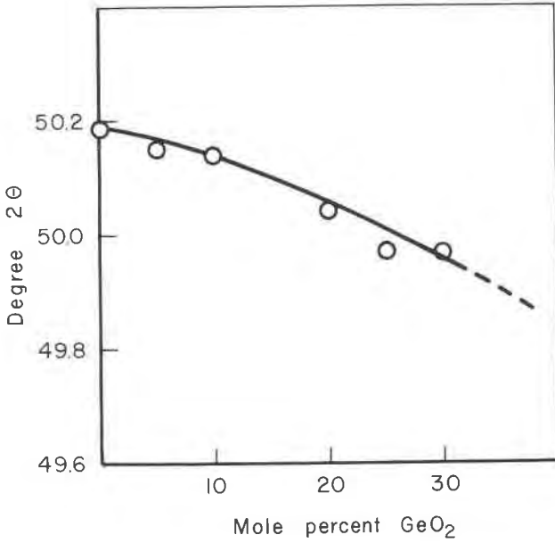
FIG. 1. Change of quartz (ss) (112) in terms of 2\theta (CuK \alpha )
