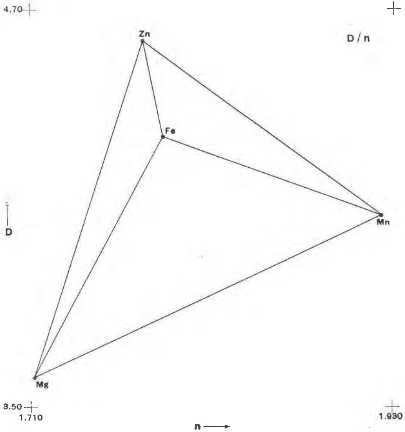
FIG. 2c. Density plotted against refractive index for the \text{Al}_2\text{O}_4 series of spinels.
