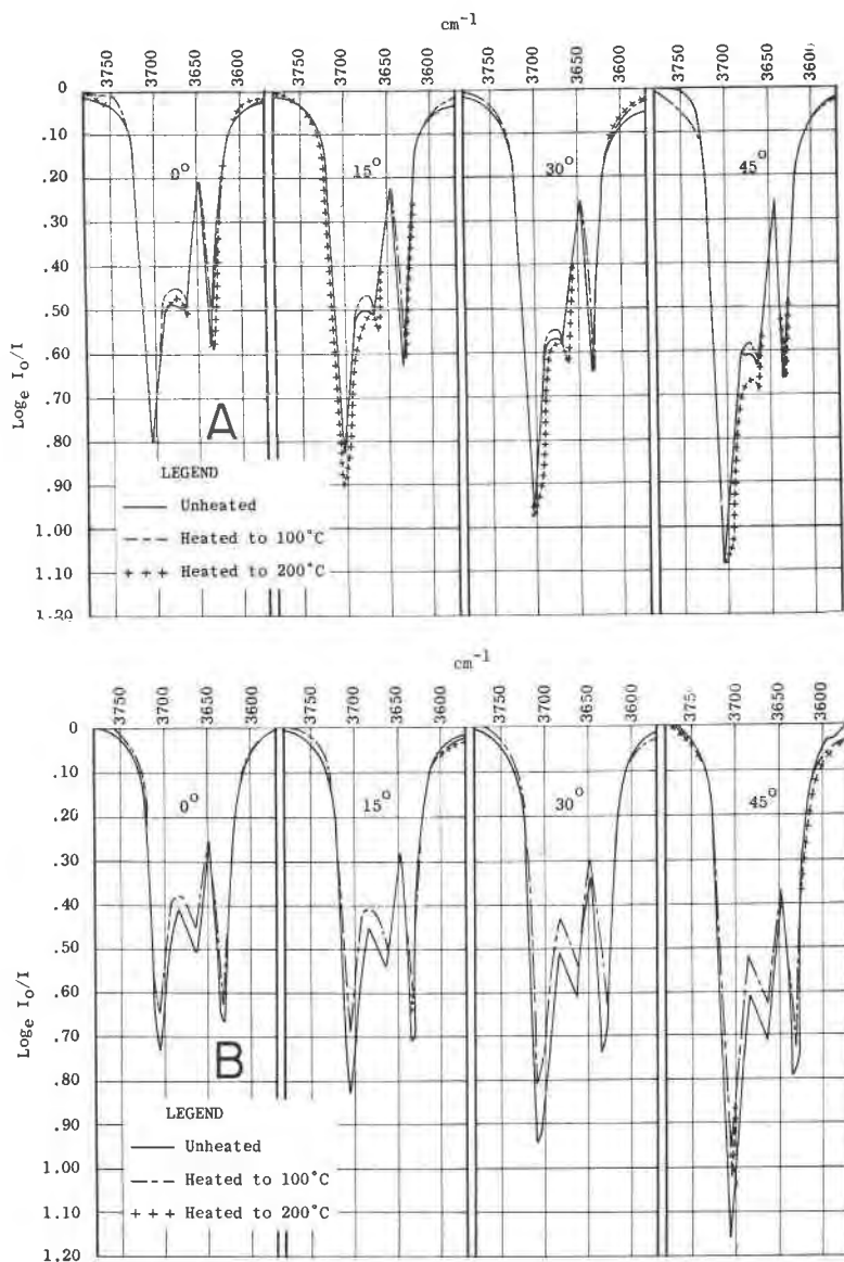
FIG. 3. Infrared absorption spectra of kaolinites (degree values refer to angle of incidence). A. Kaolinite #1. B. Kaolinite #2 (due to instrumental failure the 200^\circ\text{C} . spectra for 0^\circ and 30^\circ are not available).
