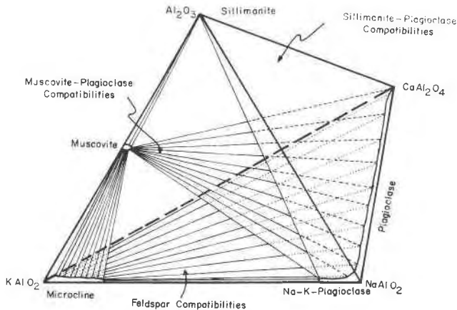
FIG. 4. Tetrahedron showing compatible minerals in the system \text{Al}_2\text{O}_3\text{-KAlO}_2\text{-NaAlO}_2\text{-CaAl}_2\text{O}_4 , in the sillimanite grade of metamorphism. Note that the assemblage muscovite-plagioclase completely cuts out the assemblage sillimanite-microcline.
