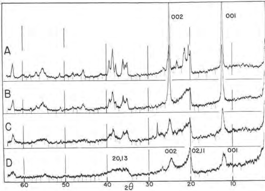
Fig. 1. X-ray powder diffraction patterns of monomineralic kaolin minerals. (A) Well-ordered, well-formed platy material, enhanced basal reflections (kaolinite). (B) Platy material with b -axis disordered sequence, enhanced basal reflections (disordered kaolinite). (C) Layer sequence partially disordered with respect to both a - and b -axes, little enhancement of basal reflections, rolled forms (halloysite). (D) Highly disordered layer sequence, no enhancement of basal reflections, tubular form (halloysite).
