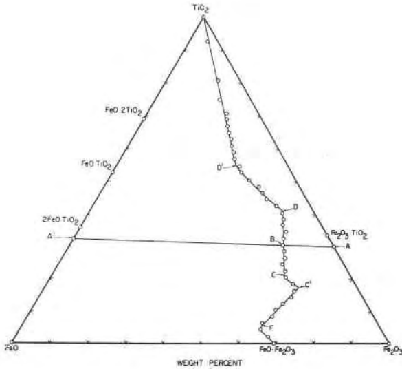
FIG. 1. Principles of the experimental method illustrated by the line which connects all compositions in the iron-titanium-oxygen system which are in equilibrium with \text{CO}_2 at 1300^\circ\text{C} . (an oxygen pressure of 10^{-3.43} atm.). A mixture of \text{Fe}_2\text{O}_3 and \text{TiO}_2 having, for example, the aggregate composition represented by point A is reduced (loses oxygen) until it has a new aggregate composition represented by point B , when heated at 1300^\circ\text{C} . in flowing \text{CO}_2 . Phase boundaries are indicated by the abrupt change in the direction of this line, as explained in the text.
