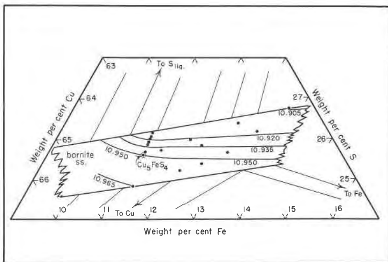
FIG. 4. Contoured plot of cell edges obtained for homogeneous compositions close to bornite in the bornite solid solution field. Dots indicate bornite compositions synthesized.
