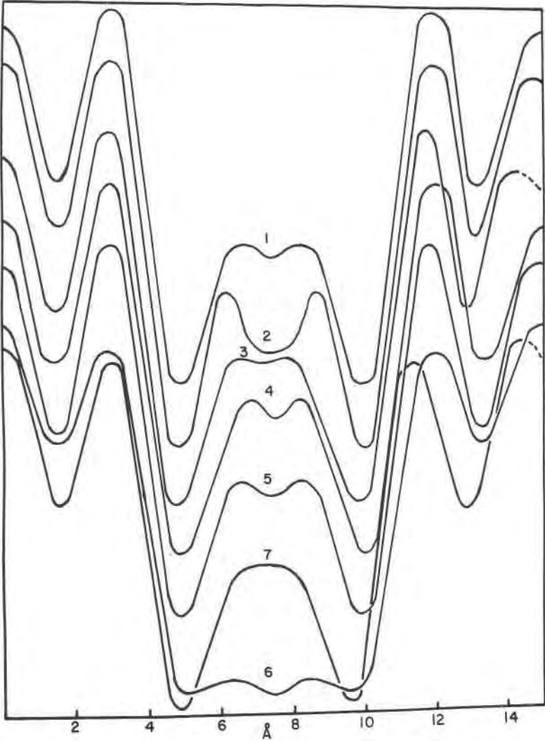
FIG. 2. Fourier curves for organo-montmorillonites calculated from x -ray diffraction data obtained at 30° C.
