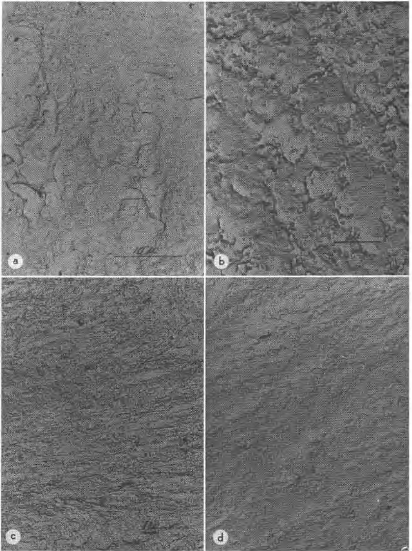
FIG. 3. Electron micrographs of chalcedony and agate.
