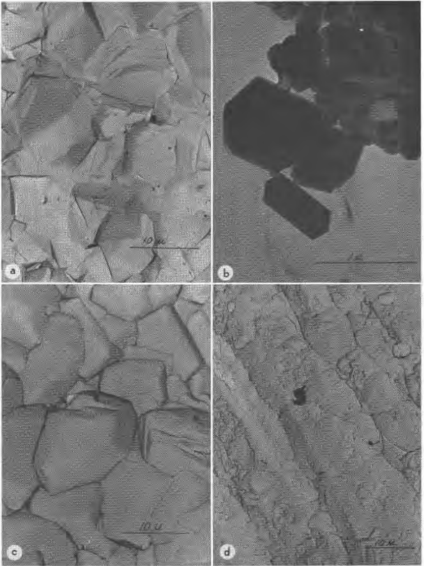
FIG. 2. Electron micrographs of jasper.
