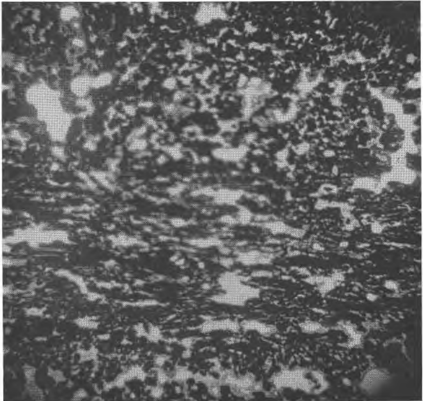
FIG. 1. Leucophosphate (light gray) lining cavities in itabirite. Diagonal of area is 5 mm.
