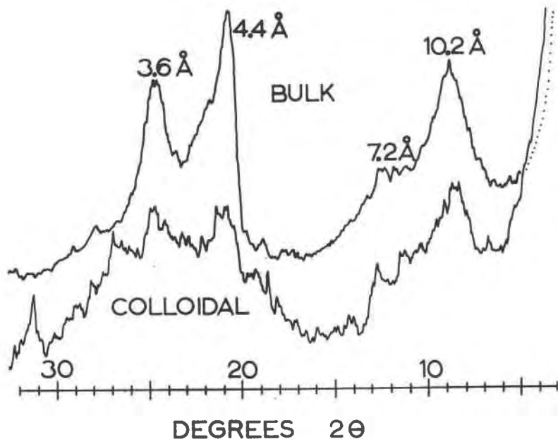
FIG. 1. Dragon Mine halloysite. The position of the 10.2 \text{ \AA} peak depended upon hydration. When heated to 400^\circ \text{ C.} for 2 hrs., a broad peak between 7 and 8 \text{ \AA} was obtained, with no peaks indicating longer d spacings. An oriented slide of the glycerated material was x -rayed using 1^\circ divergence and scatter slits, a 0.003 -inch receiving slit, 2^\circ 2\theta/\text{min.} , time constant 8, \text{CuK}\alpha , Ni filter, 40 \text{ KV} . The bulk material was run at 20 \text{ MA} , 200 \text{ counts/sec.} full scale. The colloidal material (apparently less crystalline) was run at 30 \text{ MA} , 100 \text{ counts/sec.} full scale.
