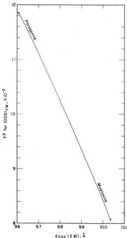
FIG. 6. Calculated F^2(006)_{2M} as a function of the d spacing of (002)_{2M} . The other stipulations are identical with those for Fig. 5.
