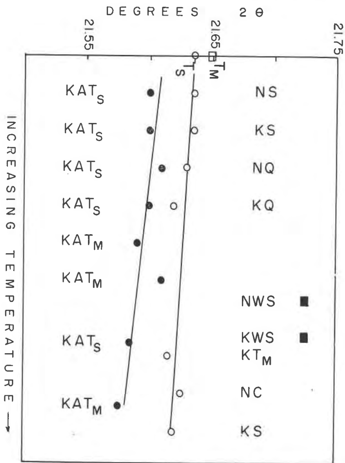
FIG. 4. X-ray spacings of tridymite samples using \text{CuK}\alpha radiation. Solid circles correspond to compositions on left, open circles and squares to compositions on right. Abbreviations same as for Fig. 2.
