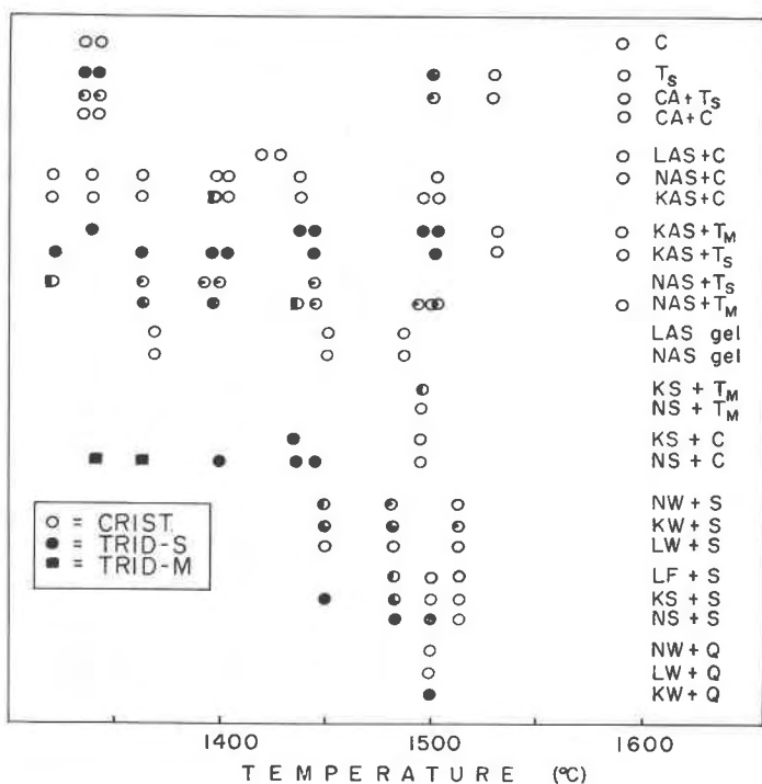
FIG. 2. Phases formed as a function of temperature by reaction of \text{SiO}_2 modifications with various fluxes. Abbreviations: C=3-C cristobalite, T_s =stable tridymite, T_m =meta-stable tridymite, CA= \text{CaO} \cdot \text{Al}_2\text{O}_3 , LAS= \text{Li}_2\text{O} \cdot \text{Al}_2\text{O}_3 \cdot \text{SiO}_2 mixtures, NAS= \text{NaAlSiO}_4 glass, KAS= \text{KAlSi}_3\text{O}_8 glass, KS= \text{K}_2\text{O} \cdot 4\text{SiO}_2 glass, NS= \text{Na}_2\text{O} \cdot 2\text{SiO}_2 glass, NW= \text{Na}_2\text{WO}_4 , KW= \text{K}_2\text{WO}_4 , LW= \text{Li}_2\text{WO}_4 , S= \text{SiO}_2 glass, Q=quartz.
