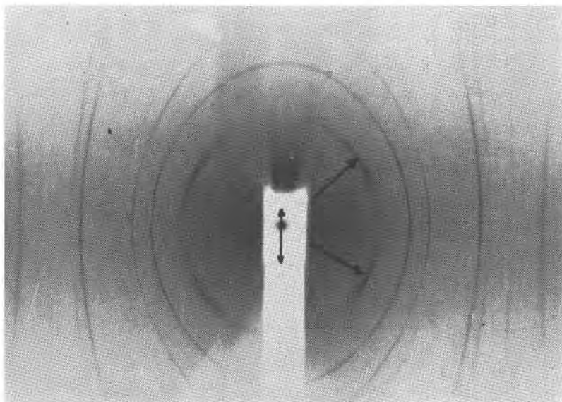
FIG. 6. X-ray pattern of a nsutite oriented along the [1\bar{1}0] and heated at 400^{\circ}\text{C} . for 21 hours. Diffuse reflections having an interplanar spacing of d=3.1 \text{ \AA} are indicated.
