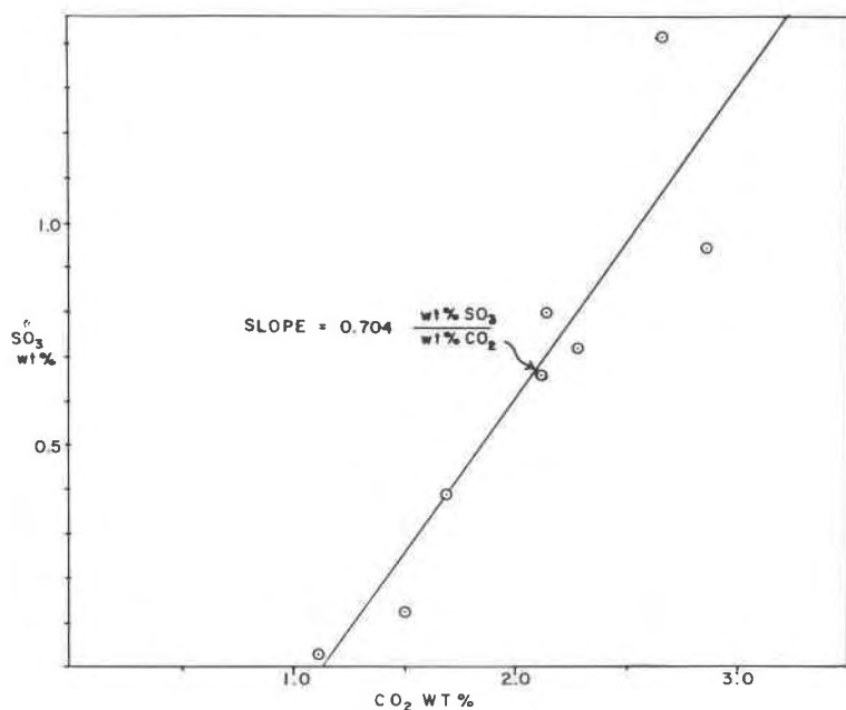
FIG. 3. Relation between \text{SO}_3 content and \text{CO}_2 content (weight per cent) in eight scapolites, based on analyses in a single laboratory.
