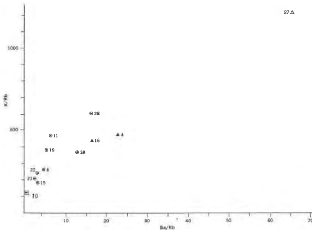
FIG. 5. K/Rb vs. Ba/Rb.
