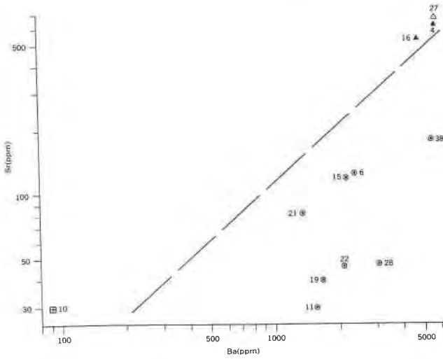
FIG. 7. Ba/Sr relationships. Broken line is trend of Norwegian alkali feldspars (Heier and Taylor, 1959b).
