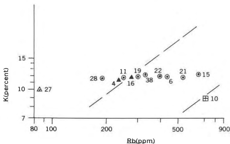
FIG. 3. K/Rb relationships. Dashed lines show "normal scatter" area (Heier and Taylor, 1959a).
