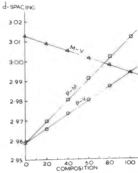
FIG. 3. Variation in 11.2 spacing with composition for synthetics of the pyromorphite series.
