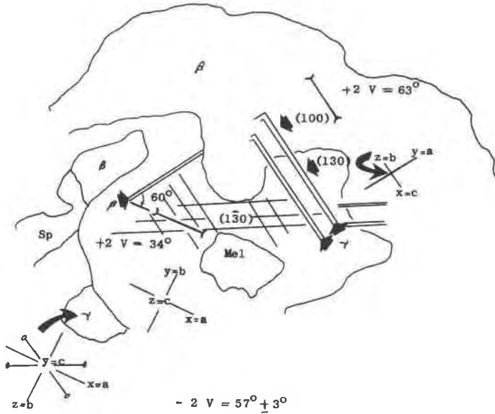
FIG. 1. Diagrams showing the orientation and crystallographic relationships between, bredigite, larnite, and \gamma in a thin section from near the contact ( \alpha' =bredigite, \beta =larnite, \gamma , Sp=spurrite, and Mel=melilite). Bredigite is oriented on the acute bisectrix. The cleavage on bredigite intersects at about 60^\circ . All patches of larnite shown on the diagram have the same orientation and are 3^\circ off center counter-clockwise in the optic plane from the acute bisectrix. The optic plane of \gamma is perpendicular to the optic plane of bredigite. Small amounts of the \gamma are present along cleavage traces in bredigite and have the orientation described above.
