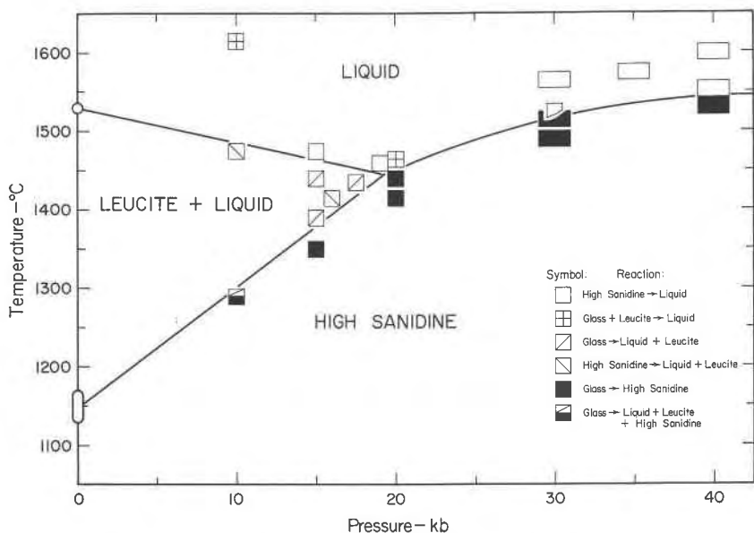
FIG. 1. Melting diagram for the composition \text{KAlSi}_3\text{O}_8 as a function of temperature and pressure. Size of symbol indicates uncertainty in temperature and pressure of each experiment. Wider symbols at 30–40 kb show greater pressure uncertainty of experiments in steel-lined bombs (see text). Symbols indicate direction of reaction but do not necessarily show complete reaction (see text). The 1 atmosphere data are from Schairer and Bowen (1955). The curve leucite + liquid = liquid is univariant only for the composition \text{KAlSi}_3\text{O}_8 ; the other two curves are truly univariant in the binary system leucite-silica.
