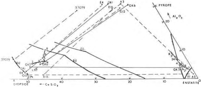
FIG. 1. Weight per cent plot of "equivalent" \text{Al}_2\text{O}_3 ( =\text{Al}_2\text{O}_3 + \text{Cr}_2\text{O}_3 + \text{Fe}_2\text{O}_3 expressed as equivalent weight of \text{Al}_2\text{O}_3 , minus the weight of \text{Al}_2\text{O}_3 equivalent to \text{Na}_2\text{O} + \text{K}_2\text{O} ) - \text{CaSiO}_3 ( =\text{CaO} expressed as equivalent weight of \text{CaSiO}_3 ) - \text{MgSiO}_3 ( =\text{sum of FeO} + \text{MnO} + \text{NiO} + \text{MgO} expressed as the equivalent weight of \text{MgSiO}_3 ). The two pyroxenes of herzolite G.K.3, the chrome diopside from Buell Park (B.P.) and the two garnet-pyroxene assemblages G.K.6 and G.R.1 are plotted and compared with (i) solvus boundary in synthetic pyroxenes in the system \text{CaO-MgO-Al}_2\text{O}_3\text{-SiO}_2 at 1600^\circ\text{C} , 30 kilobars (based on data by O'Hara, 1963c; Davis, 1963). (ii) solvus boundary in synthetic and natural pyroxenes at 1450^\circ\text{C} , 30 kilobars (based on data by O'Hara, 1963a, b; Davis, 1963), (iii) tentative solvus boundary for orthopyroxene at 50 kilobars, 1450^\circ\text{C} , estimated from data by Davis, (1963), Boyd and England, (1964), Macgregor and Ringwood, (1964), (iv) an apparent solvus boundary for clinopyroxenes from true kimberlite sources, (v) the mineral parageneses of some specimens from kimberlite:—the garnet peridotite A.3 (O'Hara and Mercy, 1963); the eclogite 37079 (O'Hara, 1963b); the eclogites E.4, E.16 and G.12 (Nixon et al. , 1963) and (vi) the pyroxene parageneses of spinel-bearing peridotite nodules in basalts from a variety of localities, numbered according to Ross et al. , (1954) 1-4 and 7, plus a group from one locality, Dreiser Weiher, Eifel, numbered according to Frechen (1963), (with one enstatite recorded as 2' instead of the original 2).
