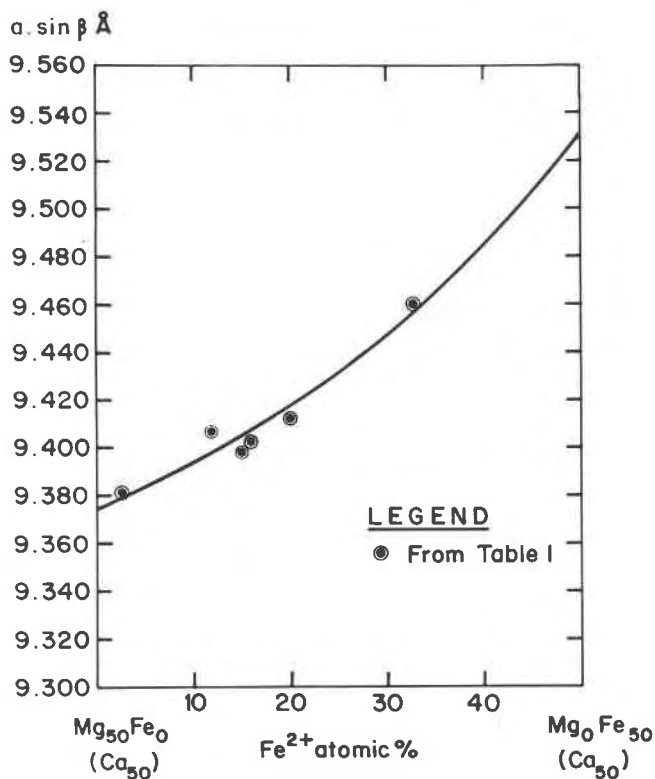
FIG. 2. Variation in the a \sin \beta dimension of the clinopyroxene unit cell with \text{Mg}^{2+}-\text{Fe}^{2+} substitution, \text{Ca}^{2+} remaining constant at the value 50.
