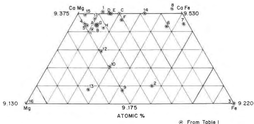
FIG. 1. The plotted points refer to the clinopyroxenes for which the analyses are given in Table 1 and the cell dimensions are given in Table 2.
