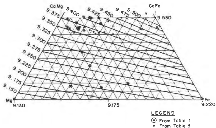
FIG. 3. Variation in a \sin \beta throughout the common clinopyroxene trapezium. The isodimensional lines for values 9.475 Å and 9.500 Å are drawn as dashed lines.
