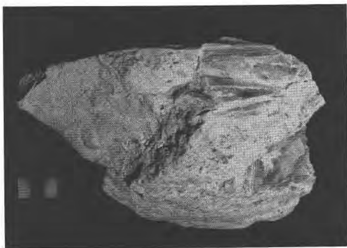
FIG. 1. Subparallel aggregates of ezcurrite crystals (upper and lower right) embedded in micro-crystalline borax surficially altered to tinalconite. Approximately one-third actual size; width of small rectangle represents one centimeter.
