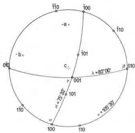
FIG. 2. Ezcurrite. Crystal drawing showing major forms.
