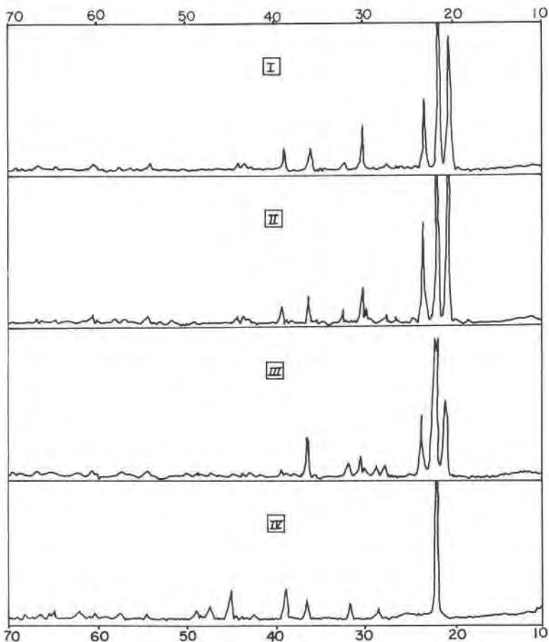
FIG. 1. Selected X-ray diffractometer patterns (Two-Theta range: 70^{\circ} – 10^{\circ} ; Radiation: \text{CuK}\alpha )—I: Tridymite-I; II: Tridymite-II; III: Tridymite-III; IV: Cristobalite formed from Tridymite-I after 16 hours at 1650^{\circ}\text{C} .
