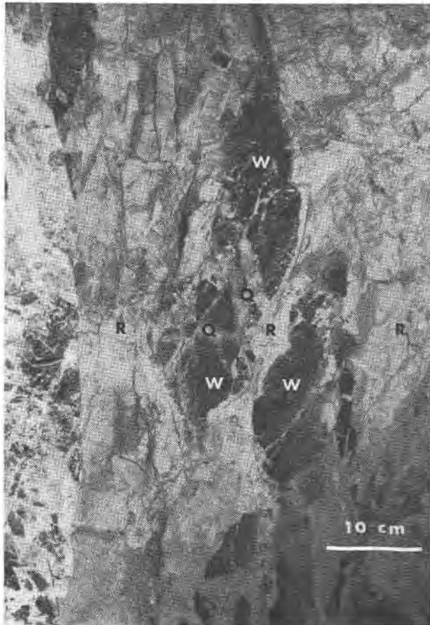
FIG. 1. A wall rock fragment (W) with stringers of quartz (Q) is surrounded by rhodochrosite (R). Ryūjima mine.
