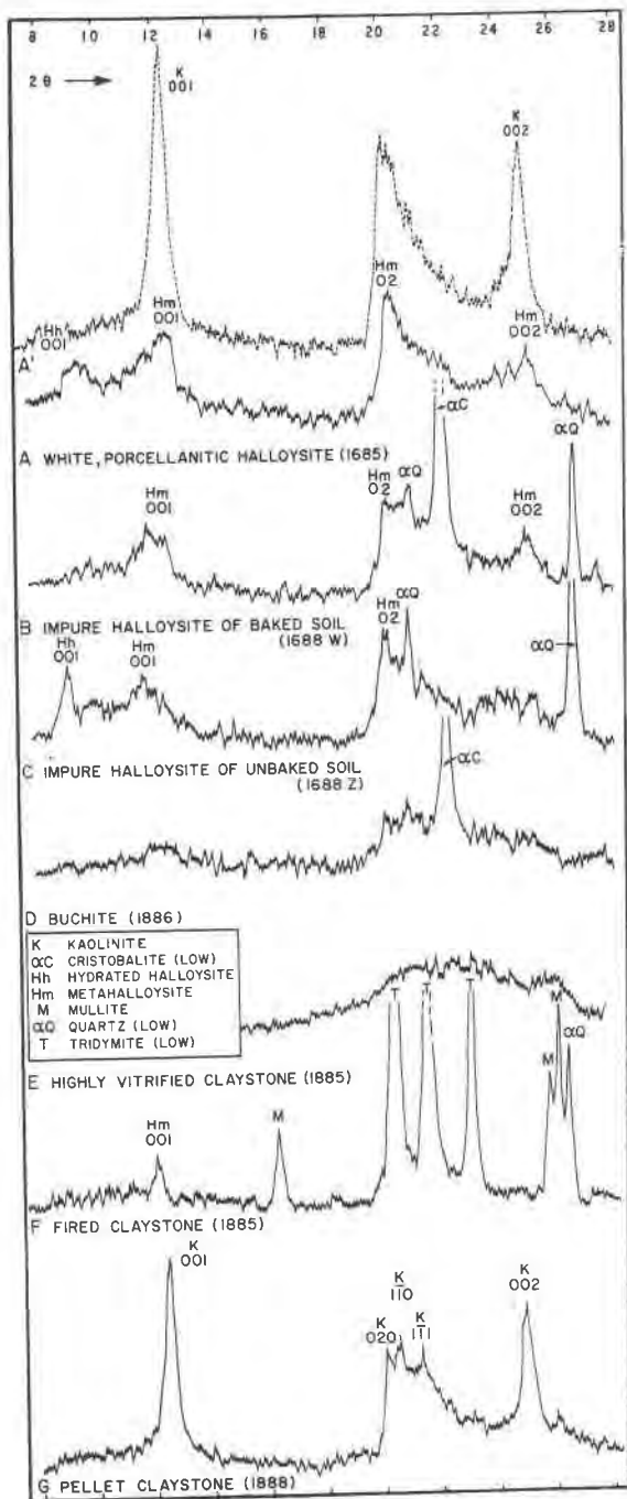
FIG. 1. X-ray diffraction diagrams of natural halloysites and their bed or host rocks. (CuK \alpha , Ni filter, Norelso instrument). The broken trace A' is for 1685 (A) heated to 300°C.
