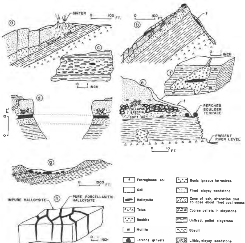
FIG. 2. Sketches illustrating the mode of field occurrence of halloysite. The scale of outcrop or specimens is of the order shown but there has been some distortion to illustrate the location of halloysite.
