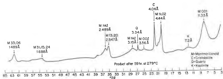
FIG. 4. X-ray diffractometer trace of an unoriented specimen of the 59 hour, 279°C sample.
