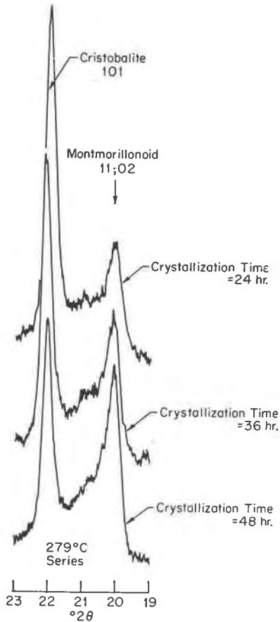
FIG. 5. Region 19 to 23° 2\theta for unoriented specimens at several reaction times.
