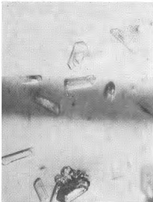
FIG. 7. Photomicrograph of phenacite inclusions in synthetic hydrothermal emerald, 400 \times .
