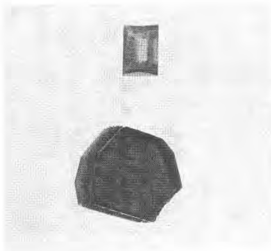
FIG. 1. Synthetic emeralds grown from Li-molybdate flux. As-grown tabular hexagonal prism crystal, 8.5 ct., 0.5% Cr. Faceted stone, lens-cut crown, step-cut pavilion, 1.13 ct., 0.09% Cr.
