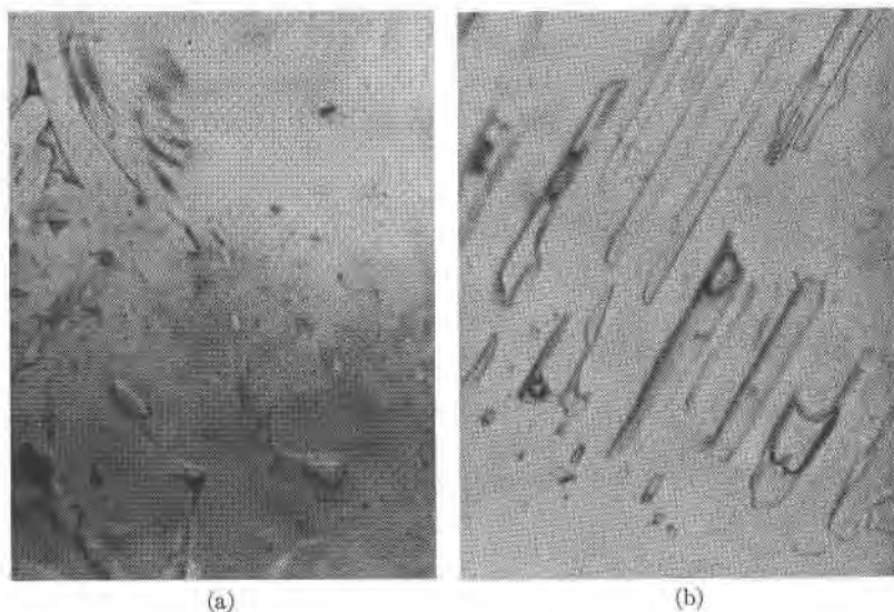
FIG. 5. Photomicrograph of 2-phase inclusions consisting of liquid and gas, in synthetic hydrothermal emerald, 400 \times . Irregular shaped voids. Elongated tube-like cavities.
