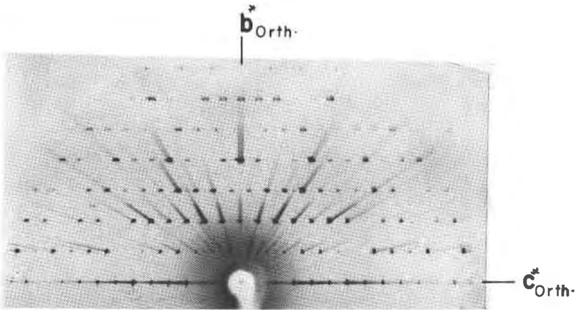
FIG. 3b. OkI precession photograph for a prehnite from Ashcroft, British Columbia. \text{MoK}\alpha , 30^\circ\mu , 50 Kv, 20 Ma, 78 hours. Orthorhombic cell; a=4.62 \text{ \AA} , b=5.48 \text{ \AA} , c=18.44 \text{ \AA} . Monoclinic cell; a=4.62 \text{ \AA} , b=5.48 \text{ \AA} , c=18.44 \text{ \AA} , \beta=90^\circ45' , twinned on [001]^* .
