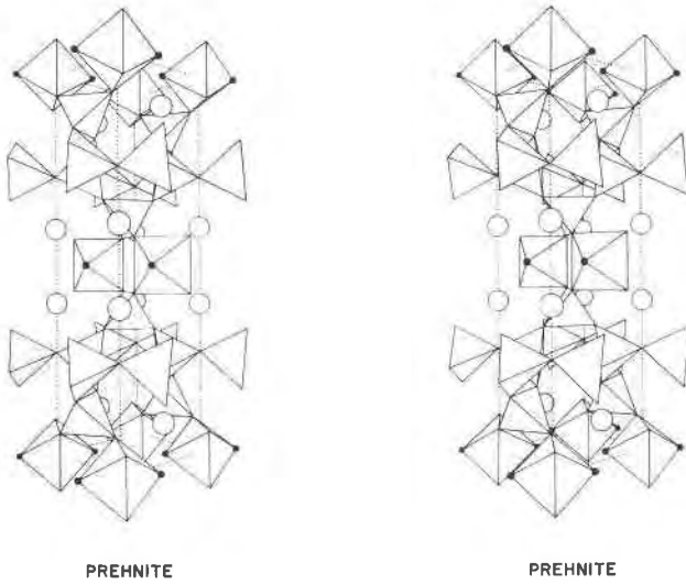
FIG. 1b. Stereographic drawing of the crystal structure of prehnite.
