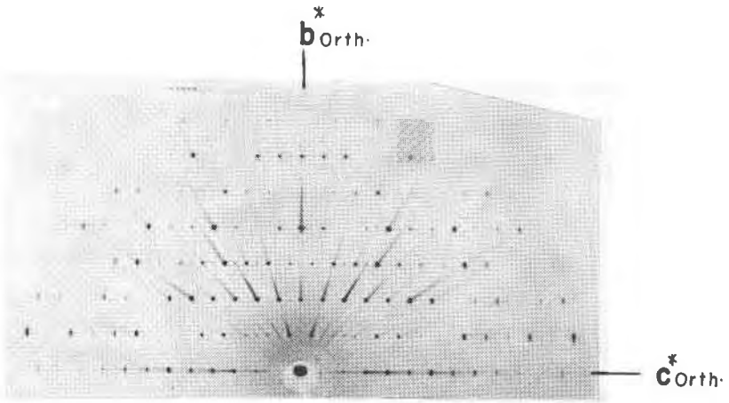
FIG. 3a. OkI precession photograph for a prehnite from Tyrol, Austria. \text{MoK}\alpha , 30^\circ\mu , 50Kv, 20 Ma, 100 hours. Orthorhombic cell; a=4.62 \text{ \AA} , b=5.47 \text{ \AA} , c=18.44 \text{ \AA} . Monoclinic cell; a=4.62 \text{ \AA} , b=5.47 \text{ \AA} , c=18.44 \text{ \AA} , \beta=90^\circ45' , twinned on [010]^* .
