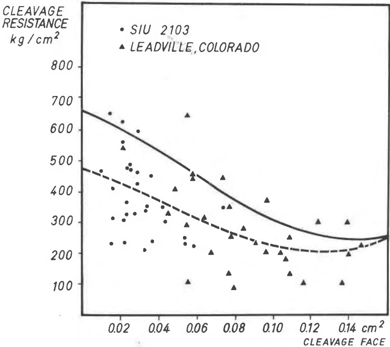
FIG. 5. Relationship between crystal size (expressed as area of cleavage face) and the cleavage resistance required by the Tertsch apparatus to produce rupture if the guillotine blade is parallel to a {100} face in pyrite. The triangles represent experimental data for cubes from Leadville, Colorado; the solid black circles represent data for pyrite labelled 2103 in the Southern Illinois University collection. The curve best fitting the combined data is represented by the dashed line; that fitting selected maximum values is represented by the solid line.
