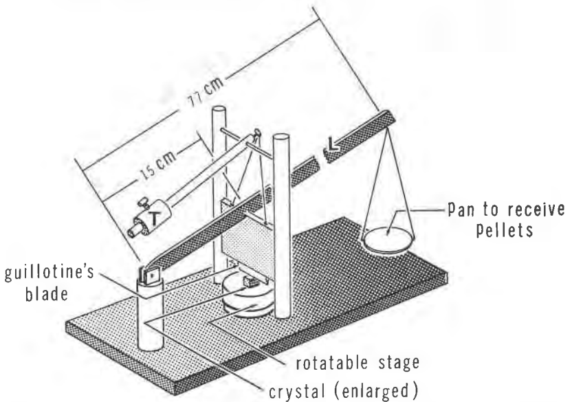
FIG. 3. Schematic diagram of Tersch's apparatus for measuring resistance to cleavage along particular directions in a crystal.
