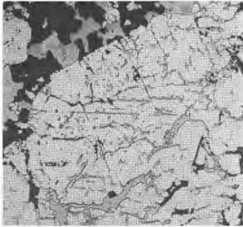
FIG. 2. Penetration of bournonite (gray) along the \{100\} cleavage directions in pyrite (white) as shown in a polished, random section for a Mine George specimen. ( \times 165 , reflected light).
