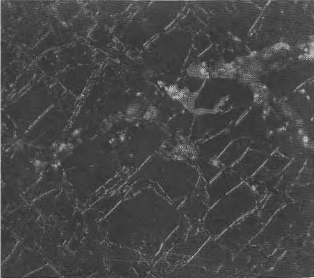
FIG. 1. Typical cubic cleavage in pyrite as shown in a polished section parallel to (100) for pyrite from Mine George near Horhausen, Siegerland, W. Germany. ( \times 165 ; dark field illumination).
