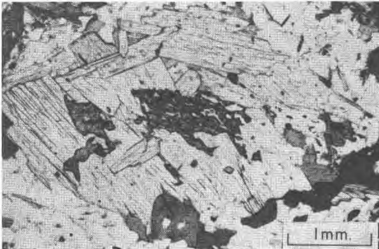
FIG. 2. Early stages of muscovite pseudomorphism: (A) Incipient muscovite plates forming around staurolite, (B) Coarse muscovite plates completely rimming remnant staurolite grains. Note sharp grain boundaries.
