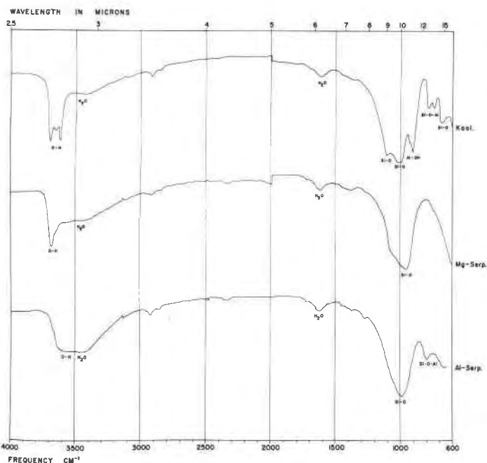
FIG. 2. Infrared spectra of a kaolinite, an Mg-serpentine (from former Rock Analysis Laboratory of the University of Minnesota) and the Al-serpentine of the present study at 22°C.
