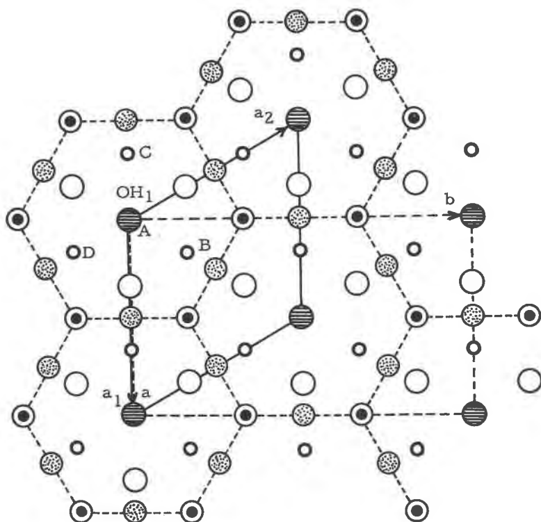
FIG. 3. c -axis projection of an idealized serpentine layer. A, B, C, D refer to the respective location of the origin of layers in the 9-layer unit cell. (Symbols: dot Si, Al; small circle Mg, Al; large circle \text{OH}_2 ; dashed circle \text{OH}_1 ; dotted circle \text{O}_{\text{basal}} ; circle over dot \text{O}_{\text{apical}} ).
