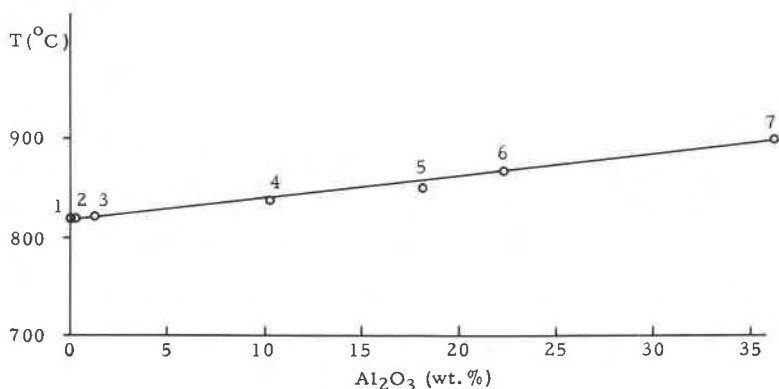
FIG. 6. Chart of the decomposition temperature and Al content of seven serpentines. (1) Orthoantigorite (Brindley and Knorring, 1954) (2) (3) Analyzed Mg-serpentines from the former Rock Analyses Laboratory of the University of Minnesota (4) Synthetic Al-serpentine (Roy and Roy, 1952) (5) Synthetic Al-serpentine (Yoder, 1952) (6) Hexagonal Al-serpentine of this study (7) Amesite (Brindley et al. , (1951).
