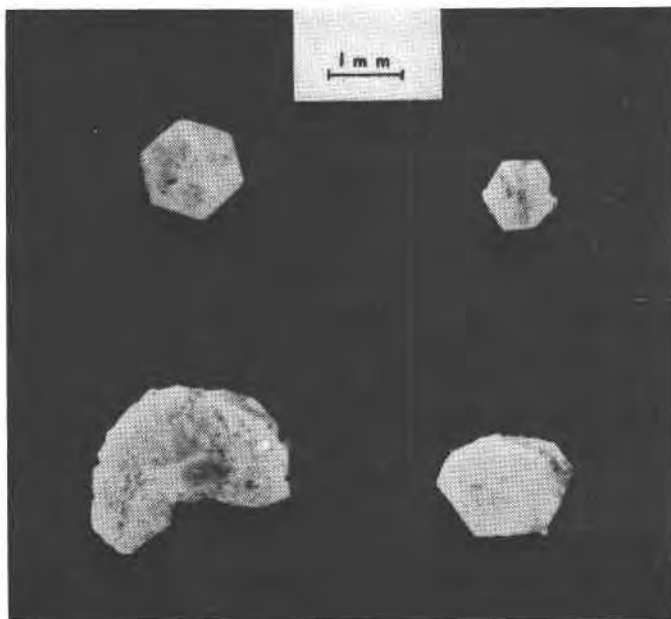
FIG. 1. Photomicrographs of Al-serpentine crystals.
