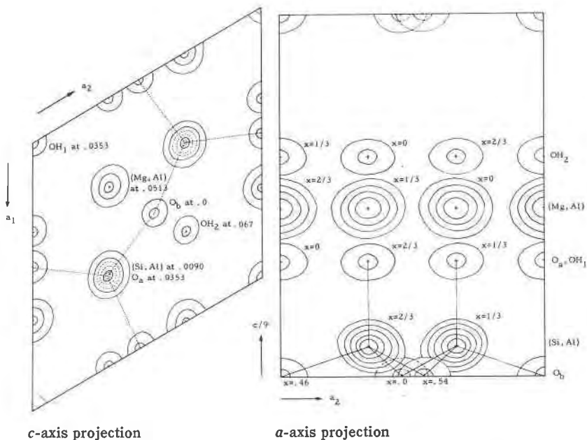
FIG. 4. c -axis projection of three-dimensional electron density sections of the first layers of the Al-serpentine structure.
