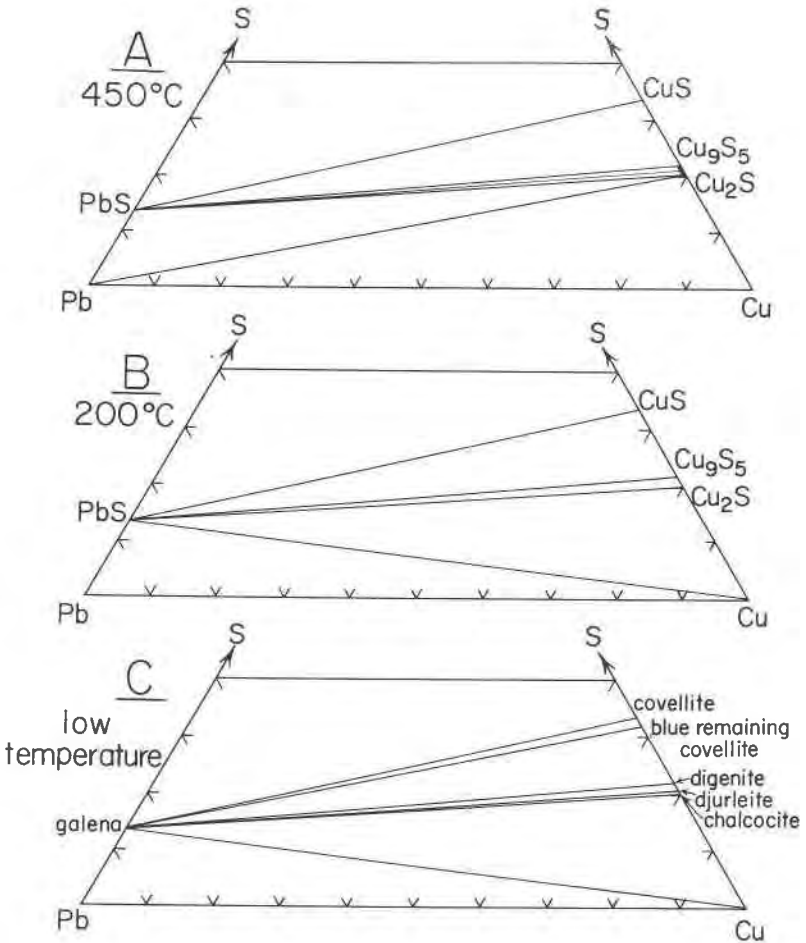
FIG. 6. Phase relations in the condensed Cu-Pb-S system at (A) 450°; (B) 200°C (note that the Cu 2 S-Pb assemblage stable at 450°C has broken down to give PbS+Cu); and (C) low temperature, as observed in ores.
