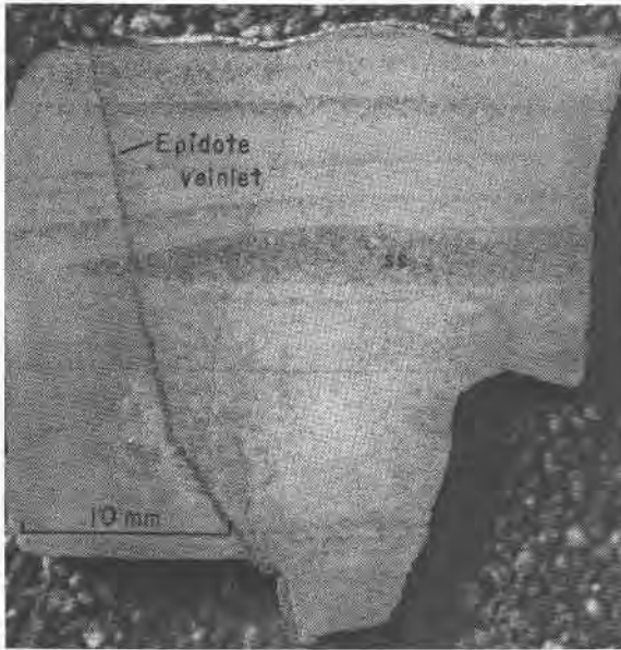
FIG. 2. Veinlet of epidote cutting metasilstone with lenses of metasandstone in W747h, I.I.D. No. 1 well, Salton Sea geothermal field. Disseminated idioblastic crystals of epidote and pyrite occur throughout the sample and are concentrated in the metasandstone lenses (ss).
