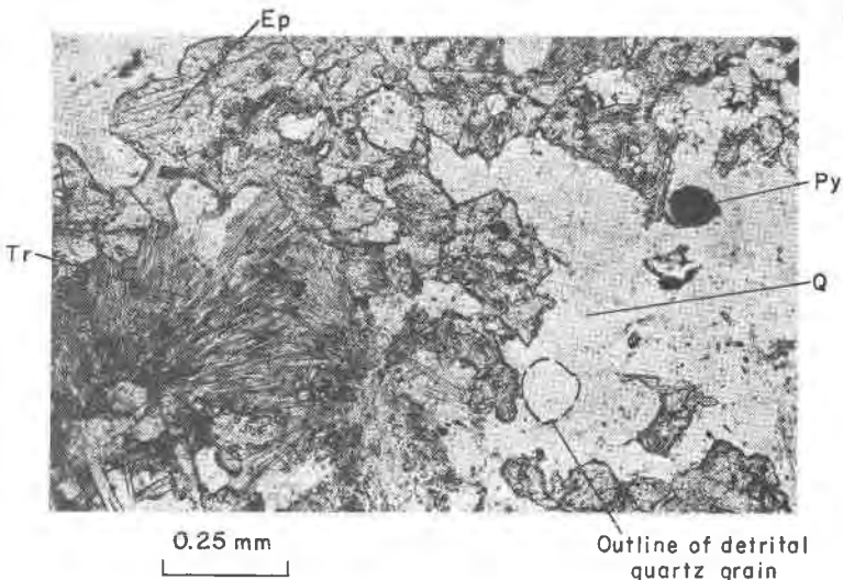
FIG. 1. Photomicrograph of metasandstone W823-4,296 from I.I.D. No. 2 well, Salton Sea geothermal field. Ep, epidote. Tr, tremolite. Py, pyrite. Q, quartz. Relict detrital form of quartz grain indicated by dashed line.
