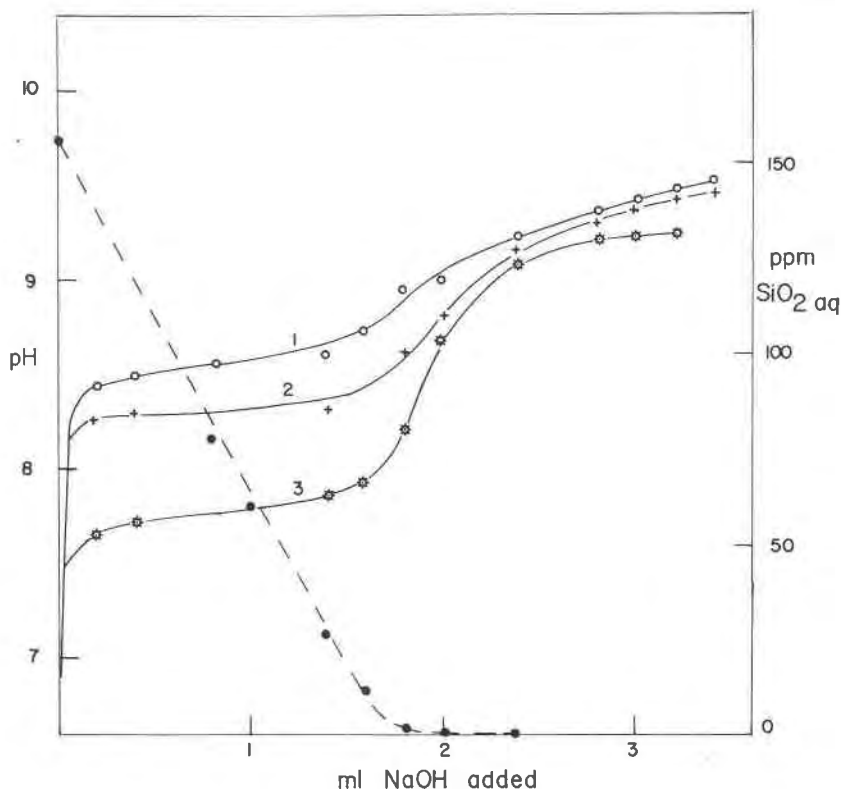
FIG. 3. Titration curve for addition of 0.10 M NaOH to a 0.1 M MgCl 2 solution containing 140 ppm SiO 2aq initially. 1, after one hour. 2, after 26 hours. 3, after 15 days. Dashed curve shows ppm SiO 2aq after 15 days.
