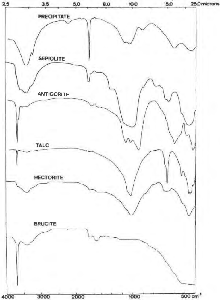
FIG. 1. Infrared absorption spectrum of the product precipitated from sea water by addition of sodium metasilicate compared with the spectra of some natural magnesium silicates and brucite. The spectra were obtained from KBr disks with a double-beam spectrophotometer.
