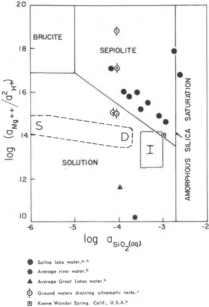
FIG. 4. Activity diagram for a portion of the system MgO-SiO 2 -H 2 O at 25°C, unit activity of H 2 O, and one atmosphere total pressure. The positions of the stability field boundaries were calculated from thermodynamic data (Hostetler, 1963; Rossini, et al. , 1952), the free energy of formation of sepiolite obtained in this paper, and are consistent with an amorphous silica solubility of 115 ppm (Morey, Fournier, and Rowe, 1964). The various symbols represent water analyses plotted as functions of \log m_{Mg^{2+}}/a_{H^+}^2 and \log a_{SiO_{2(aq)}} from: (a) Saline lake water pH values calculated from total HCO 3 - and assumed equilibrium with atmospheric P CO 2 = 10 -3.6 atmospheres. (b) River, Great Lakes and Keene Spring data from Livingstone, D. A., 1963. (c) Ground water data from Barnes, I., La-Marche, Jr., V. C. and Himmelberg, G., 1967. The areas labeled S, D, and I represent the composition of surface, deep, and interstitial sea water respectively.
