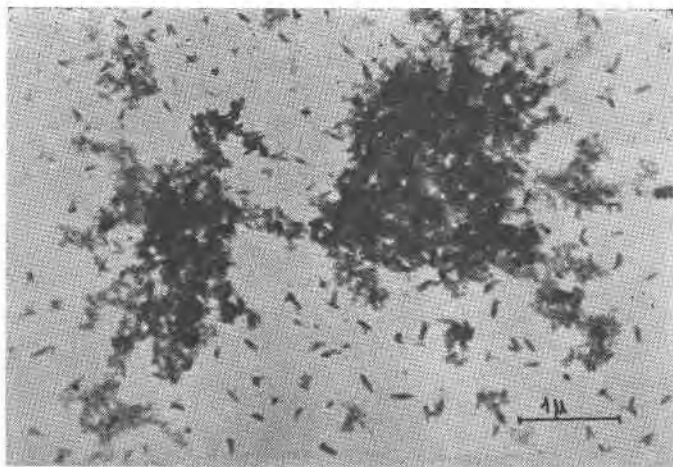
FIG. 2. Electron micrograph of synthetic sepiolite precipitated from sea water by addition of sodium metasilicate. Precipitate consists of packets of needle-shaped crystals about 0.2–0.3 \mu in length.
