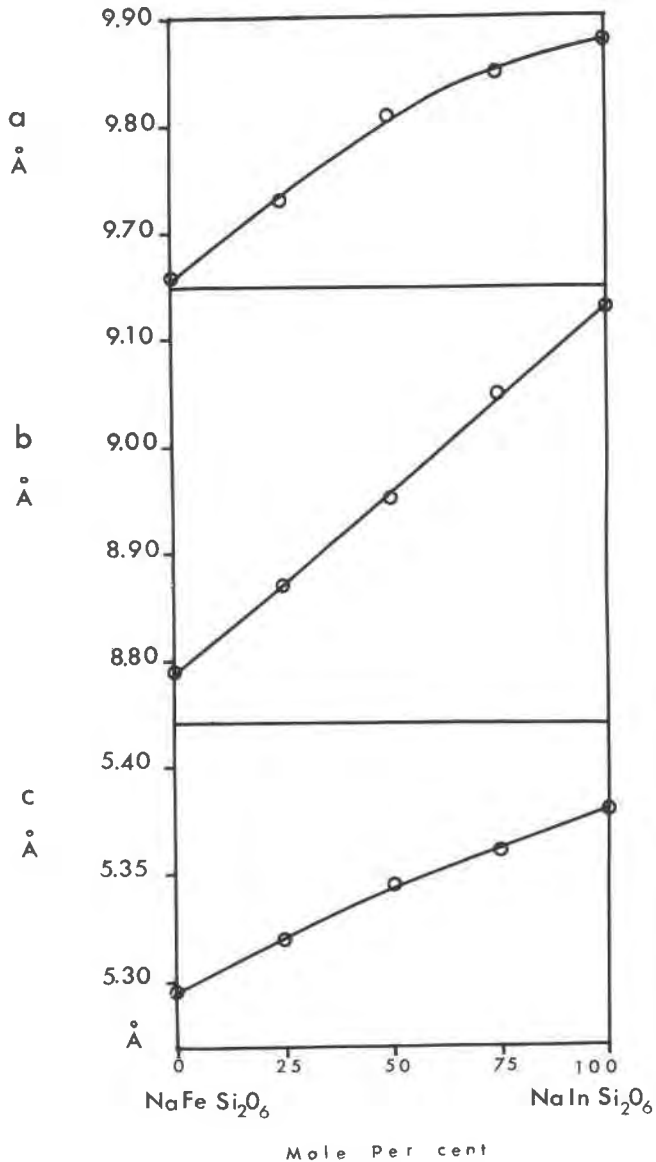
FIG. 2. Unit-cell dimensions for solid-solution series of NaFeSi 2 O 6 -NaInSi 2 O 6 .
