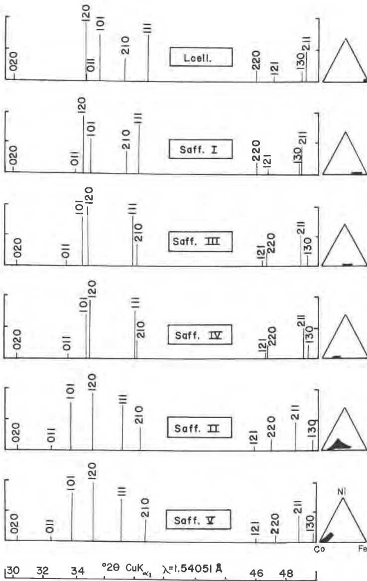
FIG. 8. 2\theta versus intensity (ordinate) for natural safflorites.
