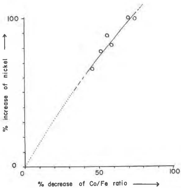
FIG. 5. Nickel content of zoned safflorites.
