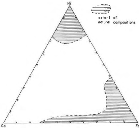
FIG. 2. Extent of natural phases, according to Holmes (1947).
