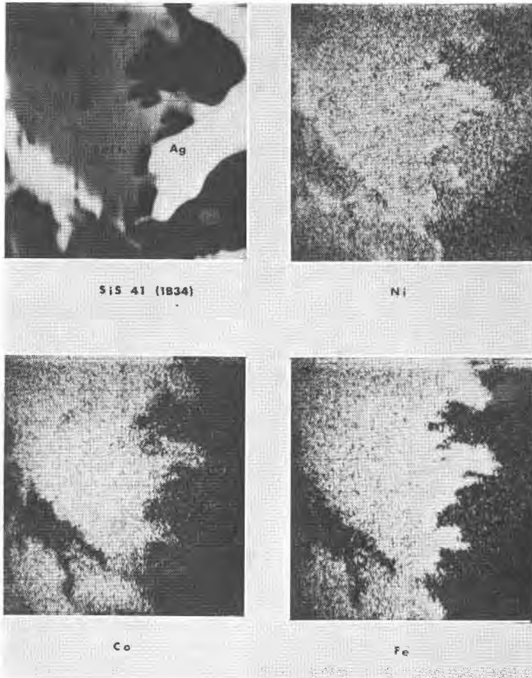
FIG. 7. Top left: Electron image of safflorite and native silver which replaces calcite (black). Top right: X-ray image showing the distribution of Ni in safflorite. Nickel is concentrated at the margins of safflorite in contact with both silver and calcite. Note the presence of some Ni in native silver. A spot check gave 0.3% Ni in this silver. Bottom: X-ray images of Co and Fe. The Co/Fe ratio decreases from left to right across both photographs and the zoning is thus different from that of Ni. Grid scale 0.03 mm.
