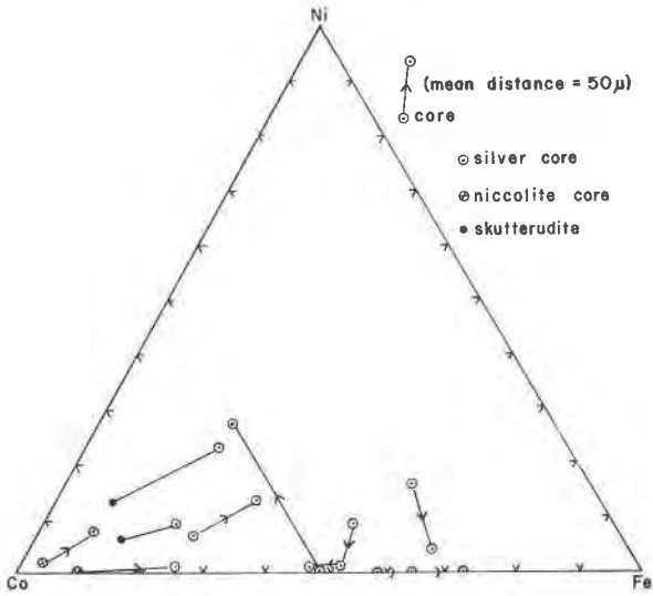
FIG. 4. Compositions of zoned safflorites. Lines with arrows represent the first seven samples of Table 3, lines without arrows the lower two samples in which safflorite and skutterudite coexist.
