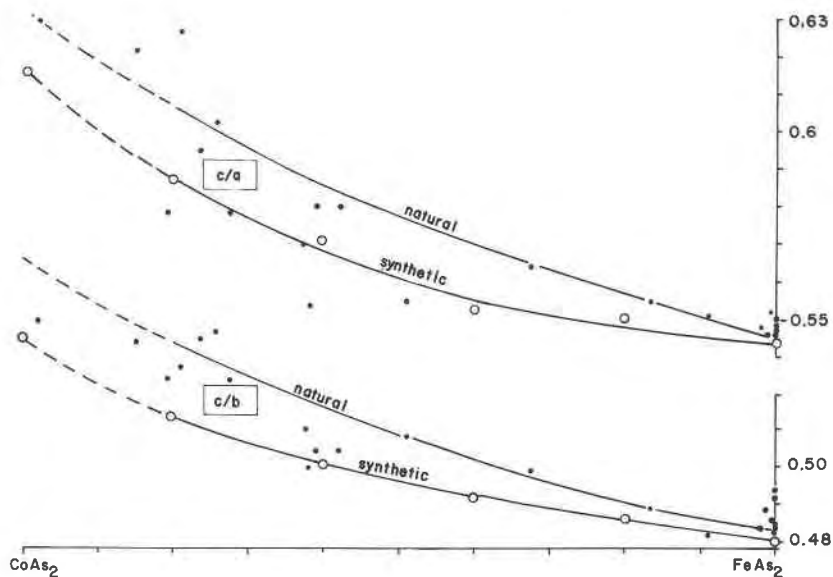
FIG. 13. Natural and synthetic safflorite. Co/Fe ratio versus c/a and c/b (loellingite-type cell).
