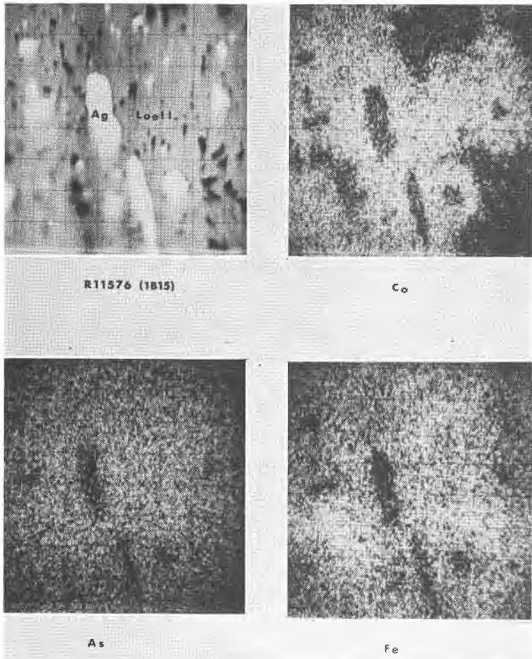
FIG. 6. Top left: Electron backscatter image of loellingite with discrete grains of native silver. Top right: X-ray scanning image showing a concentration of Co in halos surrounding native silver. Bottom left: X-ray image showing homogeneous distribution of As in loellingite. Bottom right: X-ray image showing a more heterogeneous distribution of Fe in loellingite. Grid scale = 0.03 mm.
