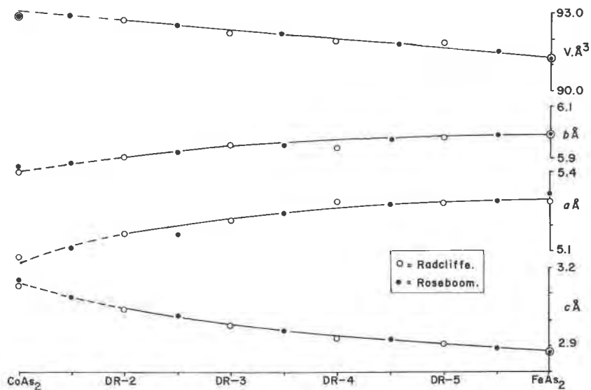
FIG. 11. Synthetic safflorites. Composition versus lattice parameters.
