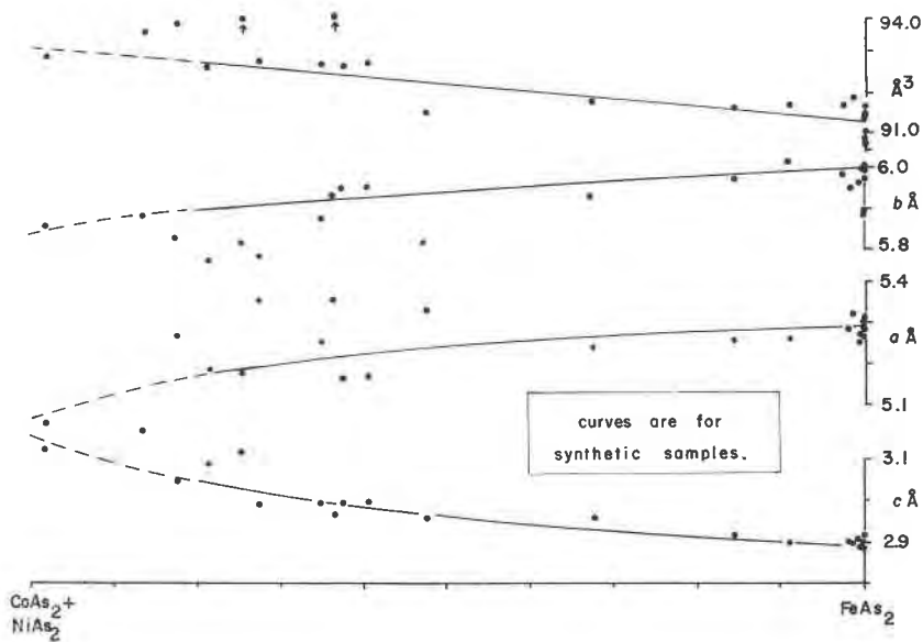
FIG. 12. Natural safflorites. Composition versus lattice parameters.
