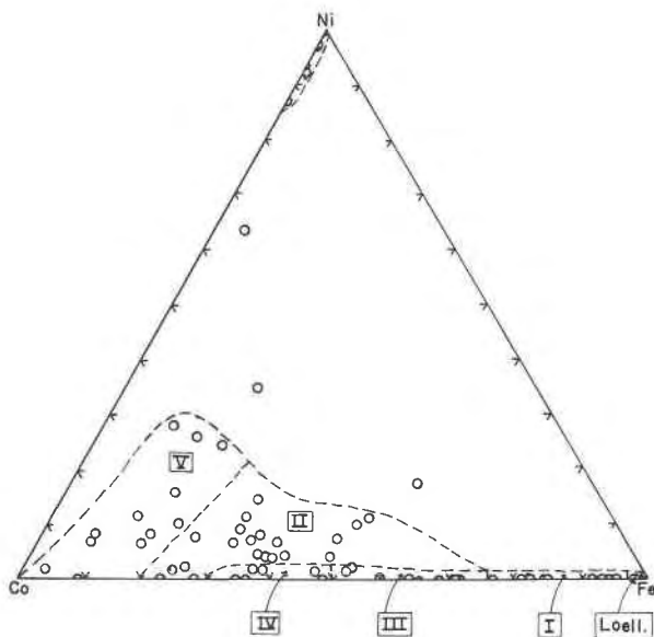
FIG. 10. Compositions of safflorite I to V.
