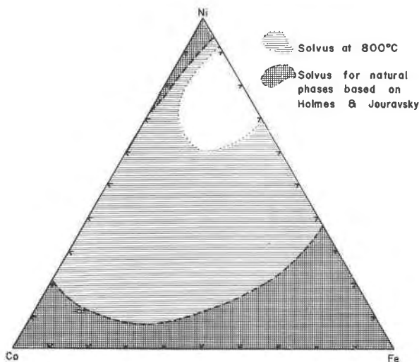
FIG. 1. Solvus for synthetic (800°C) and natural (<800°C) phases, according to Roseboom (1963).
