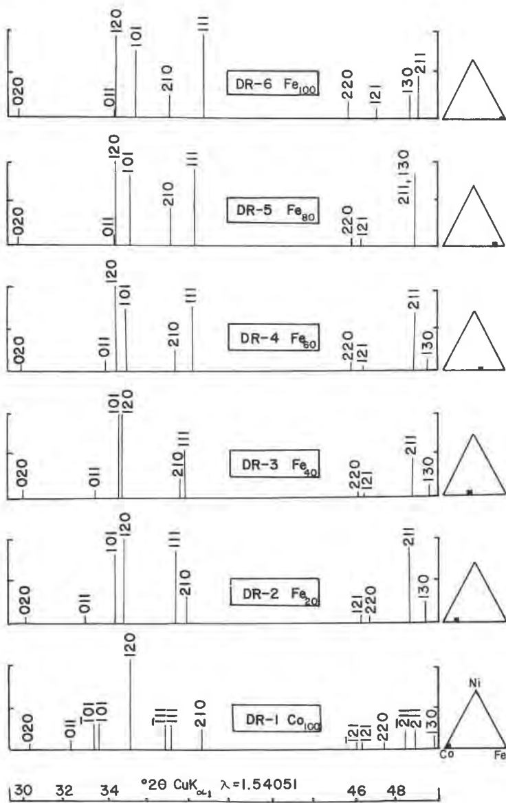
FIG. 9. 2\theta versus intensity (ordinate) for synthetic safflorites.
