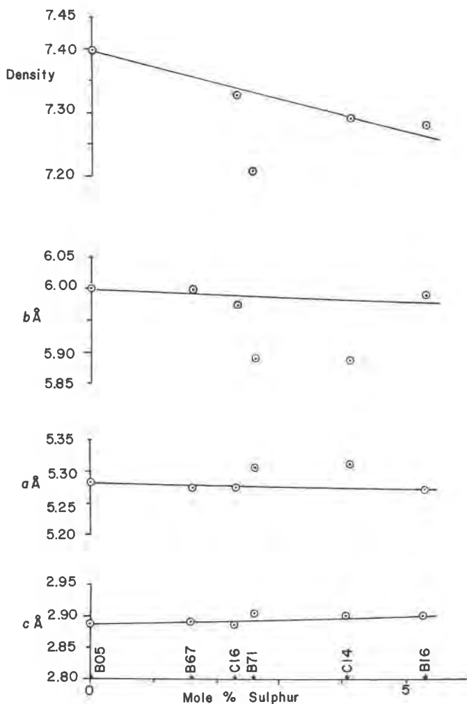
FIG. 14. Loellingite. Sulphur versus lattice parameters and density.
