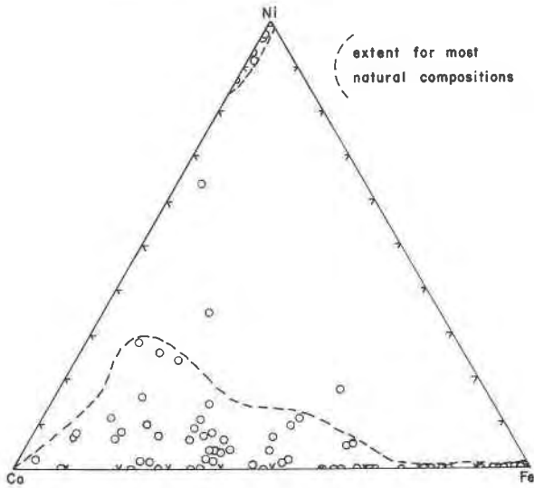
FIG. 3. Extent of natural phases analyzed in this study.
