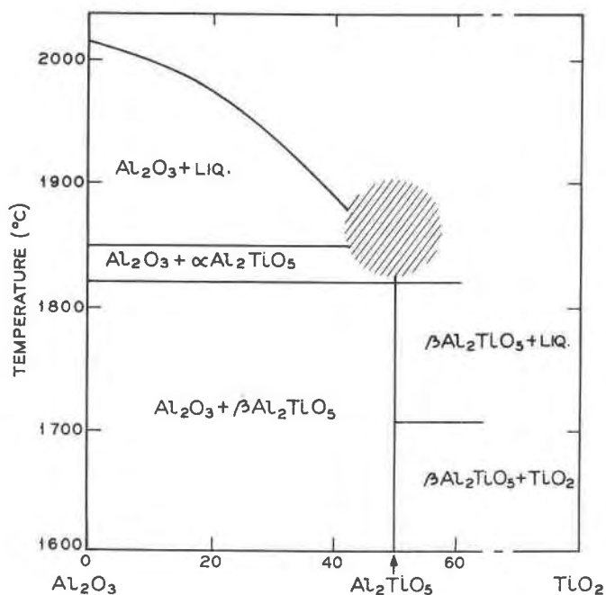
FIG. 1. Phase relations in the Al 2 O 3 :TiO 2 system after Lang, Fillmore and Maxwell (1952); uncertainties exist in the shaded region.
