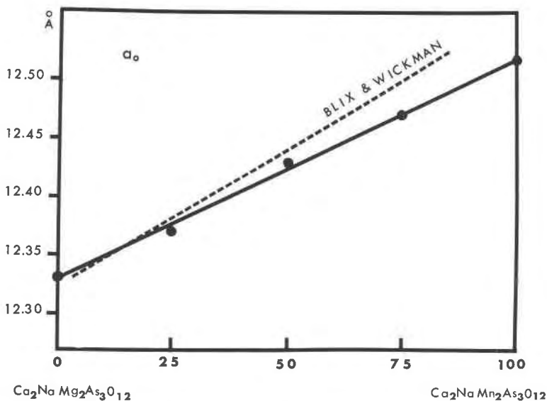
FIG. 1. Unit-cell constant a_0 of berzeliite and manganese berzeliite series.
