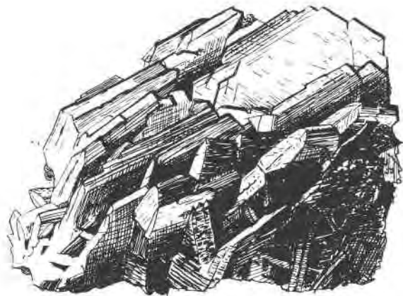
FIG. 6. Cleavelandite from Amelia.
