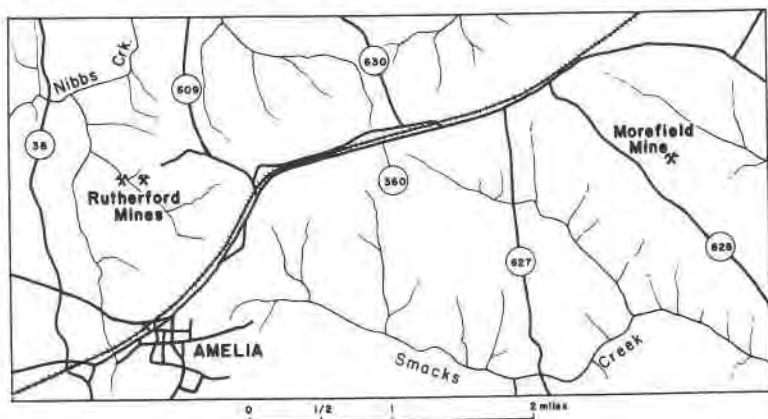
FIG. 1. Location of pegmatites near Amelia, Virginia.
