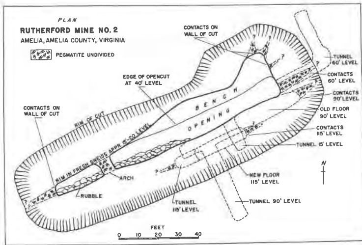
FIG. 3. Map of Rutherford No. 2 mine.
