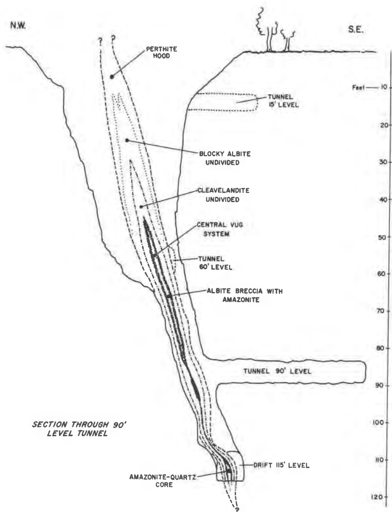
FIG. 2. Restored cross section, Rutherford No. 2 pegmatite.
