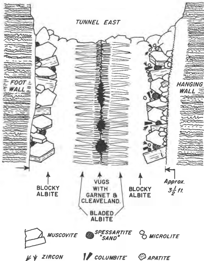
FIG. 5. Detailed cross section, Rutherford No. 2 pegmatite.
