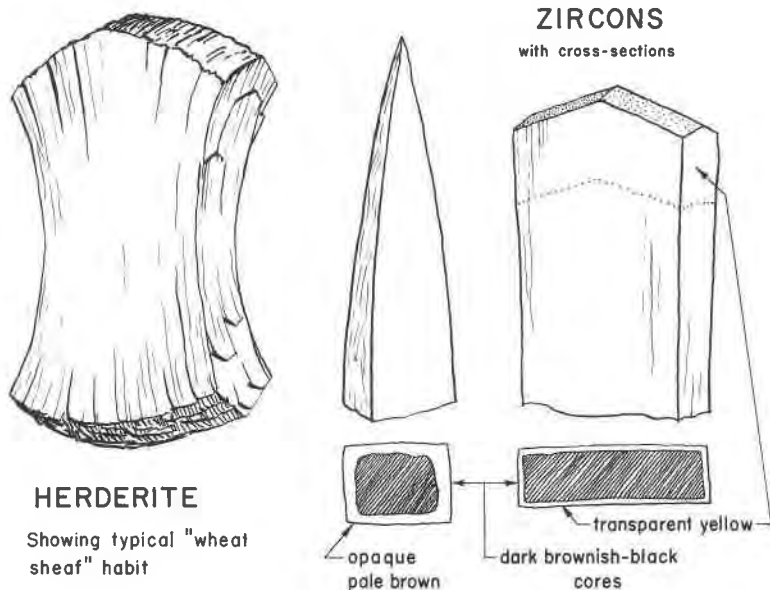
FIG. 7. Form of herderite and zircon at Amelia.
