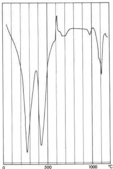
FIG. 8. Differential thermal analysis curve of bermanite from 7-U-7 Ranch, Arizona. Rate of heating 25^\circ\text{C}/\text{min.} ; reference junction 0^\circ\text{C} ; thermocouple Pt/Pt+13% Rh; reference material \text{Al}_2\text{O}_3 .
