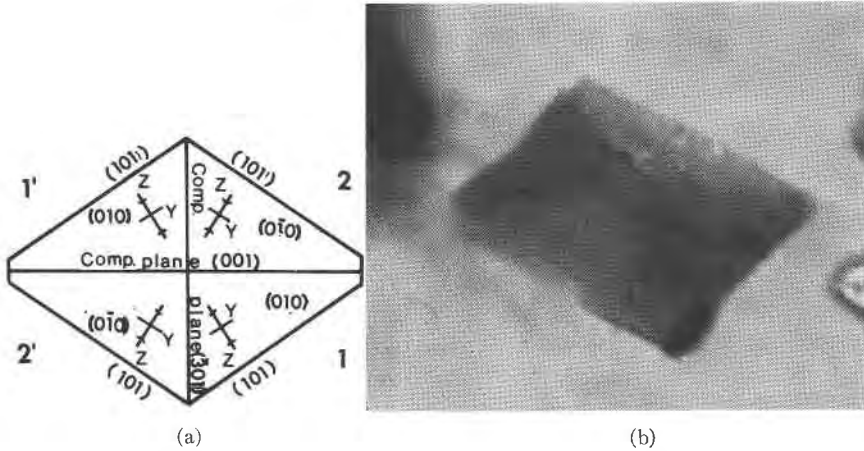
FIG. 6. Bermanite showing twins of Types 3 and 4 as seen on crystals lying on faces perpendicular to [010] . a. Drawing showing the relationship of the four individuals of the composite twin as distinguished by different optical orientations. Individuals 1 & 2, and 1' & 2' are twinned on [100] with composition plane \{001\} ; doublets 1-2 and 1'-2' are twinned on [100] with composition plane \{301\} . b. Photomicrograph showing differential absorption in differently oriented individuals. Plane polarized light, 300X.
