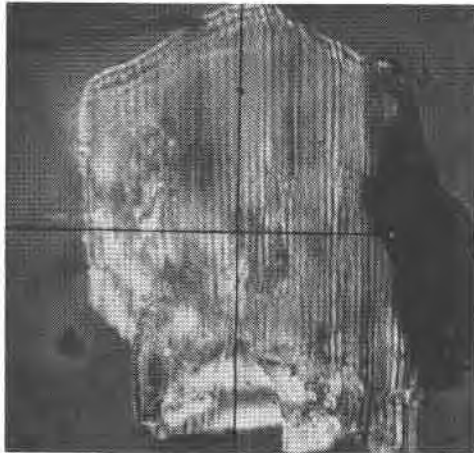
FIG. 5. Photomicrograph of bermanite showing polysynthetic twinning of Type 1. Crossed polars, 250 \times .
