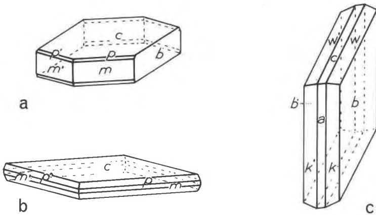
FIG 3. Crystal drawings of bermanite. a. and b. Orthorhombic orientation reproduced from Hurlbut (1936) with form lettering adjusted to conform to symmetry of point group 222. c. Crystal drawing of b in monoclinic orientation. Orthorhombic forms c , m , m' , p , p' become respectively monoclinic b and b' , a , c , k and k' , w and w' .
