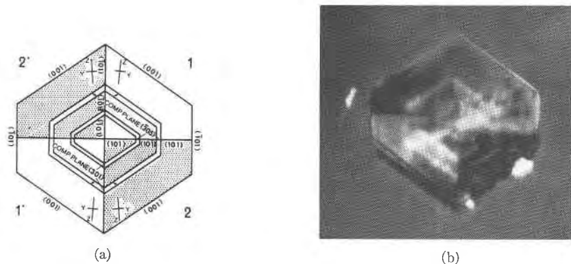
FIG. 7. Composite twin of bermanite. a. Drawing showing four major units forming a composite twin of Types 1 and 2. Each unit shows thin bands resulting from twinning of Type 3. A twin relation exists between the adjacent thin bands of quadrants 1 & 2' and 1' and 2 with composition plane \{301\} ; the plane separating the same bands between 1 & 2 and 1' & 2' is composition plane \{305\} . Since \{301\} of the thin bands is parallel to \{101\} of the thicker bands, no twin relation exists along this contact. b. Photomicrograph of twin crystals illustrated in a. Crossed nicols, 250 \times .
