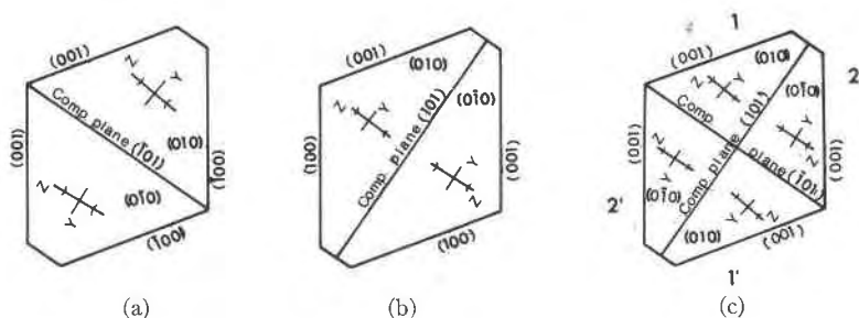
FIG. 4. Illustrations of the most common twin laws in bermanite drawn as seen lying on faces perpendicular to [010] . a. Type 1: twin axis [101] ; composition plane, \{101\} . b. Type 2: twin axis [101] ; composition plane \{101\} . c. Composite twin of Types 1 and 2.
