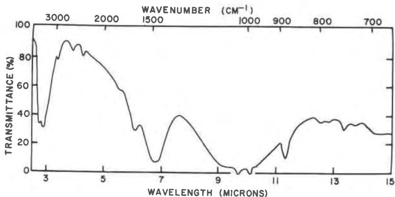
Fig. 6. Infrared absorption pattern of Mound Lake sepiolite. Perkin-Elmer Model 137 Infrared Spectrometer. KBr disc.
