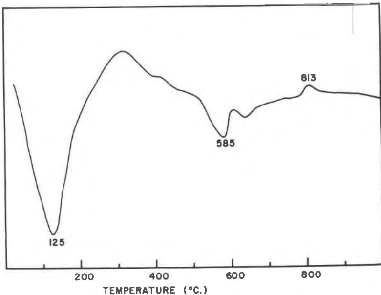
FIG. 5. Differential thermal analysis pattern of Mound Lake sepiolite. Equilibrated over saturated \text{CaCl}_2 solution, relative humidity 30%. Heating rate 12°C per minute.
