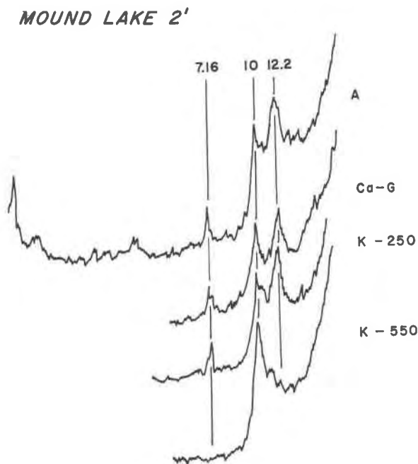
FIG. 2. X-ray diffraction patterns of Mound Lake sepiolite. A, air dried; Ca-G, calcium saturated and glycerated; K-250, potassium saturated and heated to 250^{\circ}\text{C} ; K-550, potassium saturated and heated to 550^{\circ}\text{C} . Ni filtered Cu radiation, 1^{\circ} per minute scanning speed, scale factor 4, multiplier 0.8, time constant 4.
