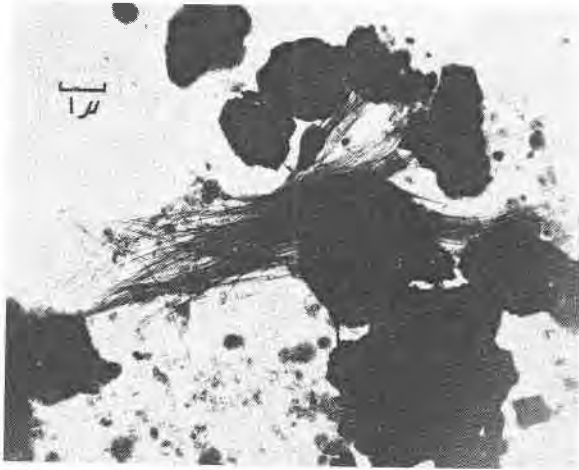
FIG. 3. Transmission electron micrograph of fibrous bundle of Mound Lake sepiolite.
