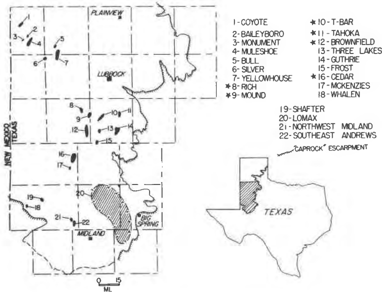
FIG. 1. Index map of pluvial lakes on the southern High Plains. Stars indicate lake basins searched for sepiolite.
