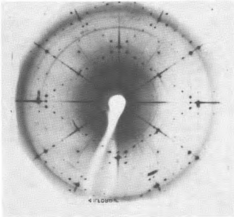
FIG. 3. Precession photograph (1\bar{1}0)_0^* of digenite, from Leonard Mine, Butte, Montana.
