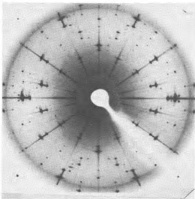
FIG. 1. Precession photograph (100)_0^* of anilite with a small amount of djurleite, from Ani Mine, Akita, Japan.
