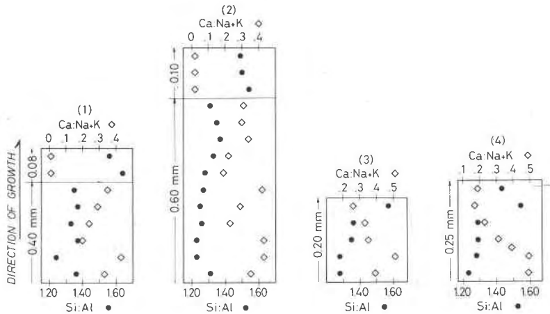
FIG. 6. Change of chemical composition within single crystal of gonardite and natrolite. The length and growing direction are shown on the left side of each figure.
