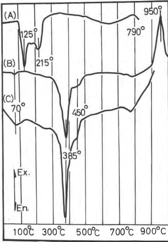
FIG. 4. DTA curves of gismondine and gonnardite. Heating rate 10^{\circ}\text{C}/\text{min.} ; reference junction 0^{\circ}\text{C.} ; thermocouple Pt/Pt+13% Rh; reference material \text{Al}_2\text{O}_3 ; in atmosphere. (A) Gismondine from Round Top, Oahu; (B) Gonnardite from Punchbowl, Oahu; and (C) Gonnardite from Maze, Japan.
