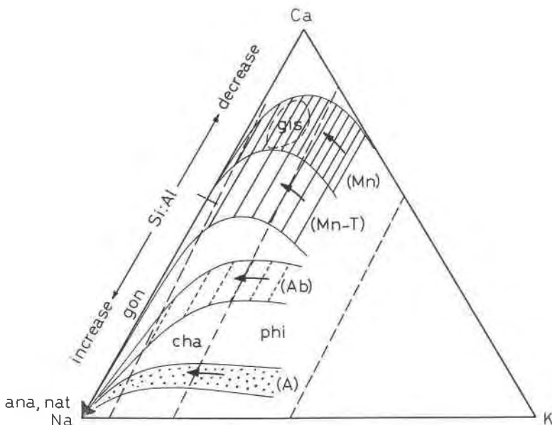
FIG. 7. Trends of the succession of authigenic zeolite formation in different types of original rocks during alteration of volcanic glass, drawn on the basis of Fig. 2. (Mn)—in melilite nephelinite tuff, (Mn-T)—in melilite nephelinite tuff containing abundant tholeiite fragments, (Ab)—in alkali basalt tuff, and (A)—in acidic tuff in saline lakes and soils. Ca:Na and Si:Al ratios of earlier-formed K-zeolites are strongly controlled by the types of original rocks. However, the final zeolite is analcime in all the tuffs.
