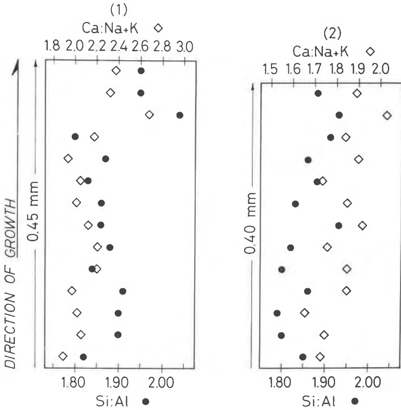
FIG. 5. Change of chemical composition within a single crystal of chabazite by electron microprobe analyses. The dimension and growing direction are shown on the left side of each figure.
