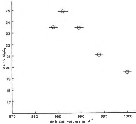
FIG. 4. Plot of the wt. % of \text{Al}_2\text{O}_3 versus the unit-cell volume for pumpellyite, from the Karmutsen Group.
