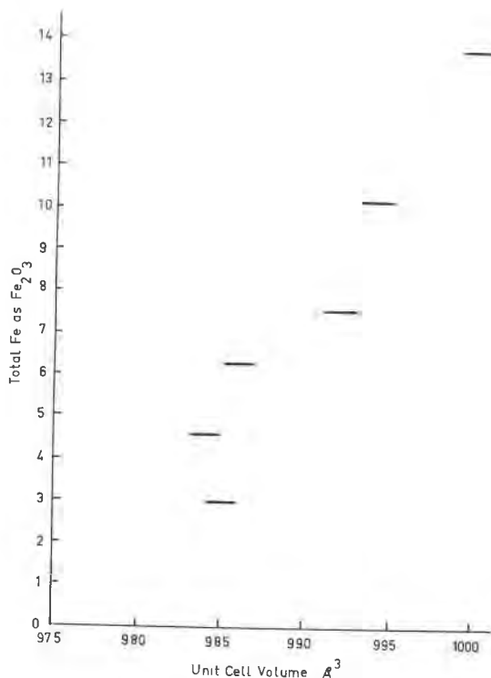
FIG. 3. Plot of the wt. % of \text{Fe}_2\text{O}_3 (total iron) versus the unit-cell volume for pumpellyite, from the Karmutsen Group.
