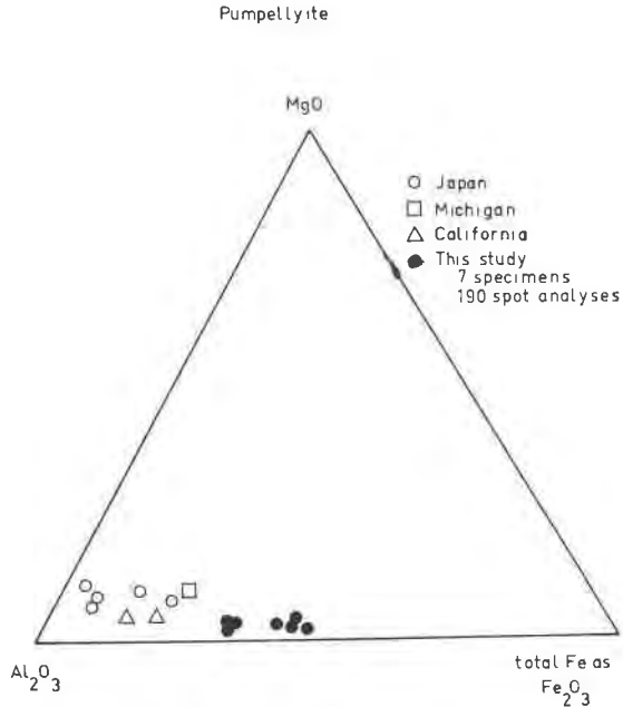
FIG. 2. \text{MgO}:\text{Al}_2\text{O}_3:\text{Fe}_2\text{O}_3 (total iron) variation diagram for pumpellyite from Japan (Seki, 1958, 1961), Michigan (Coombs, 1953), California (Coombs, 1953), and this study.
