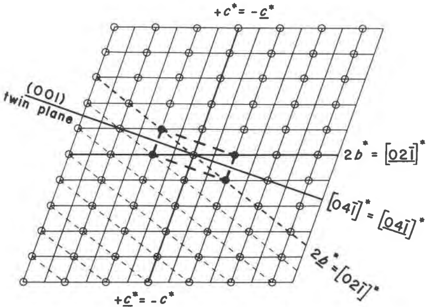
FIG. 1. Parallel twinning on (001) in chondrodite as seen on the b^*c^* reciprocal lattice plane. The vectors [021]^* and -c^* of one twin lamella (solid lines) coincide in magnitude and direction with the vectors 2b^* and +c^* of the other twin lamella (dashed); space group symmetry requires that for diffractions of the form Ok\ell , k=2n (circled). This results in the superposition of diffraction spots from both twin lamellae and a pseudo-orthorhombic cell (outlined) with b_{\text{ortho}} parallel to [041]_{\text{mono}}^* .
